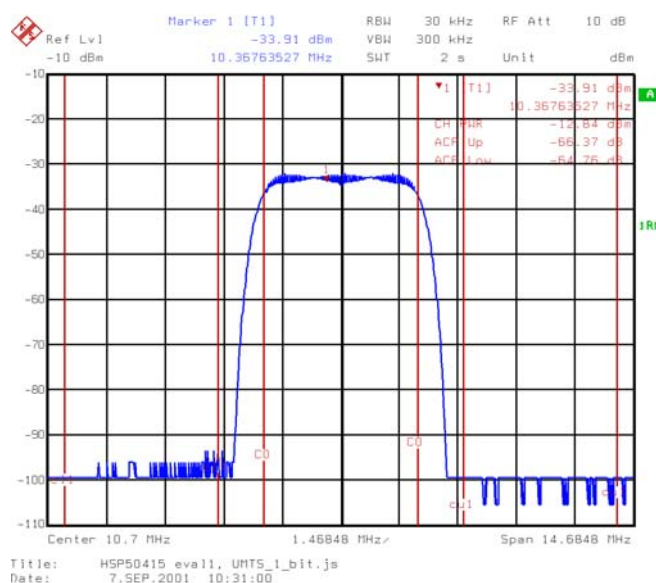
FIGURE 3. ANALOG SPECTRUM
