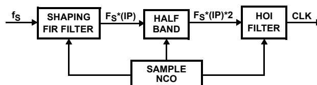
FIGURE 1. CHANNEL RATES
