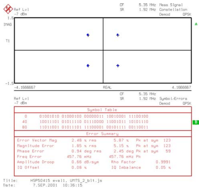
FIGURE 7. VECTOR ANALYSIS
