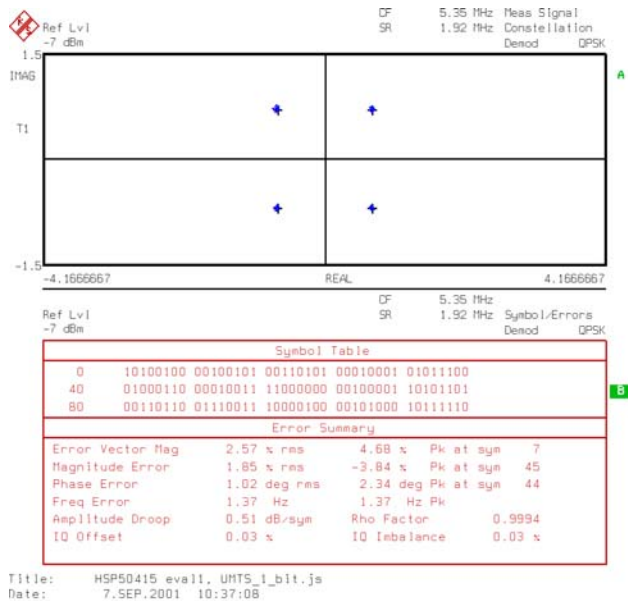
FIGURE 4. VECTOR ANALYSIS
