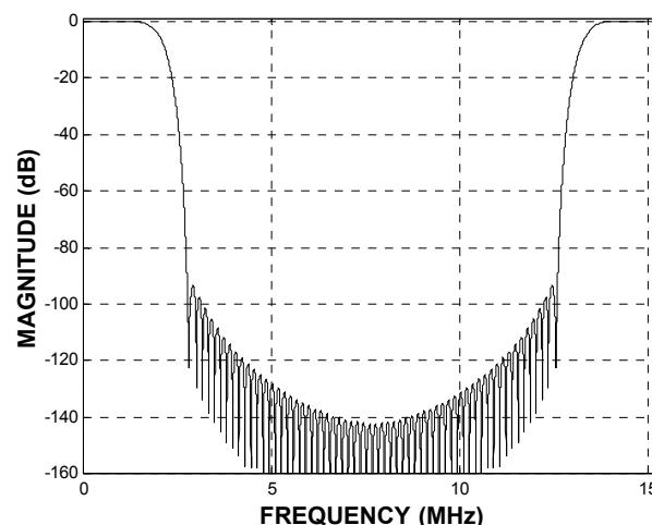
FIGURE 2. SHAPING FILTER FREQ. RESPONSE
