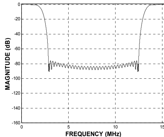
FIGURE 5. SHAPING FILTER FREQ. RESPONSE
