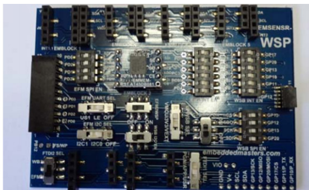
figure 3. EMSNSR Board
