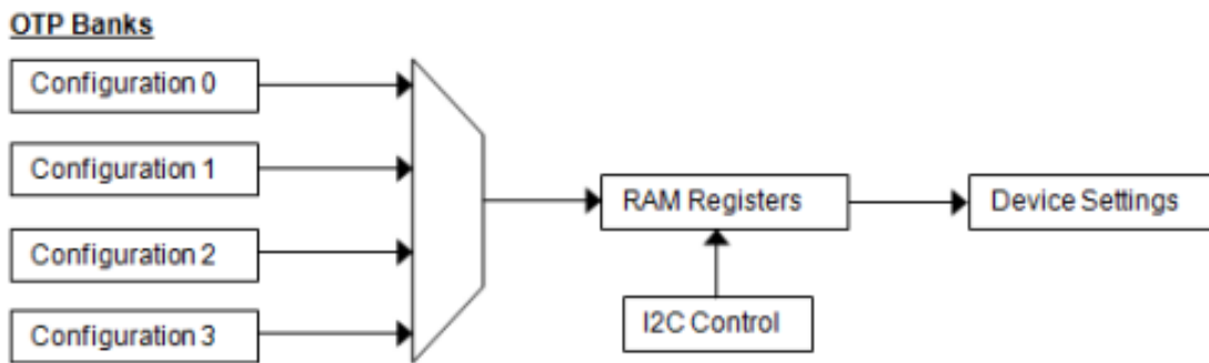
Figure 1. Register Maps
