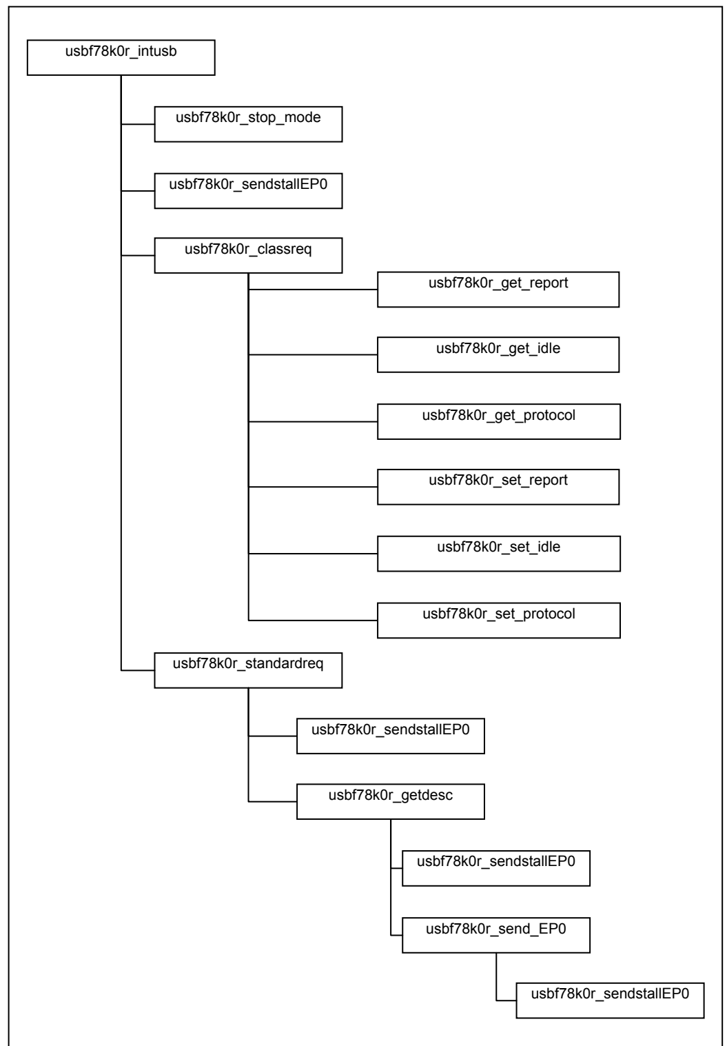
Figure 3-7 Calling Functions during the Processing for the USB function controller
