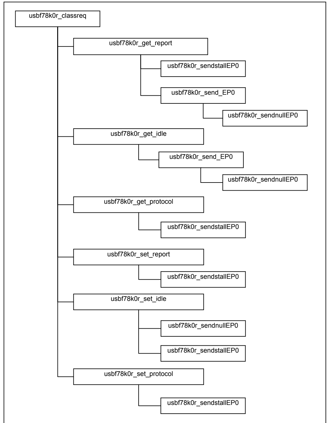
Figure 3-8 Calling Functions during the Processing for the USB HID Class (1)
