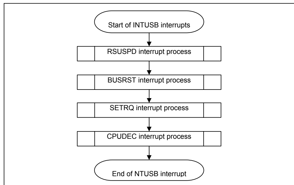
Figure 3-5 Process flow of Endpoint0 monitoring
