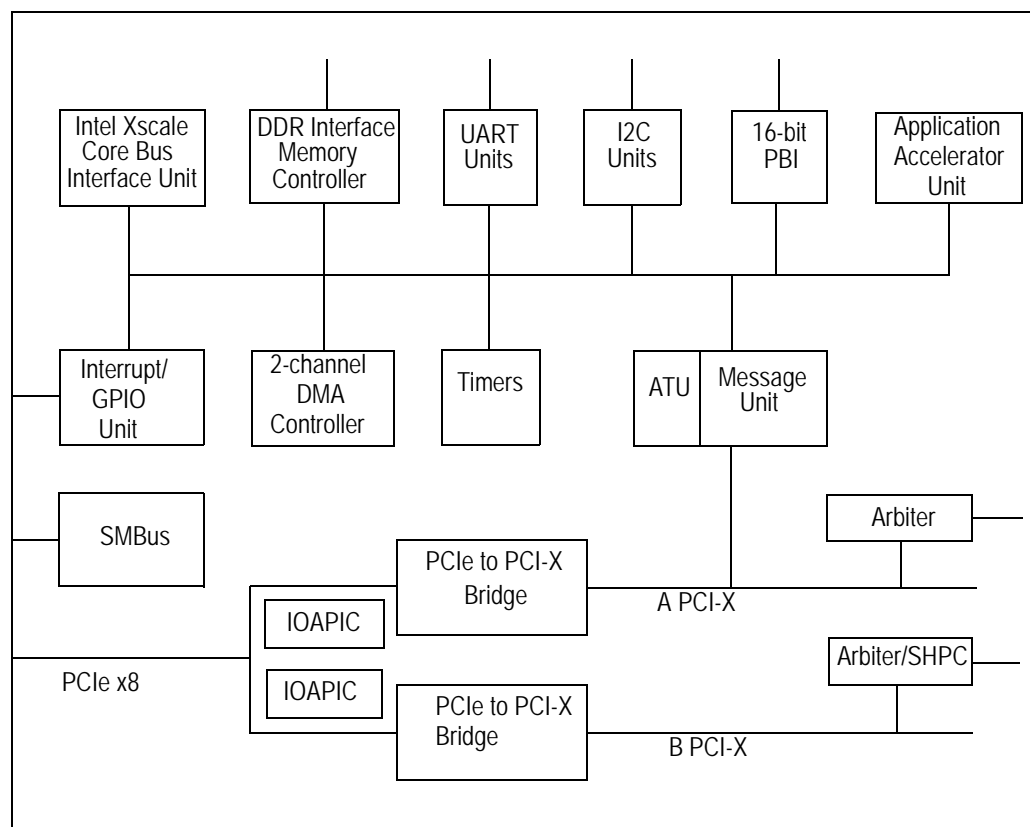
Figure 5 Intel IOP80333 Functional Block Diagram
