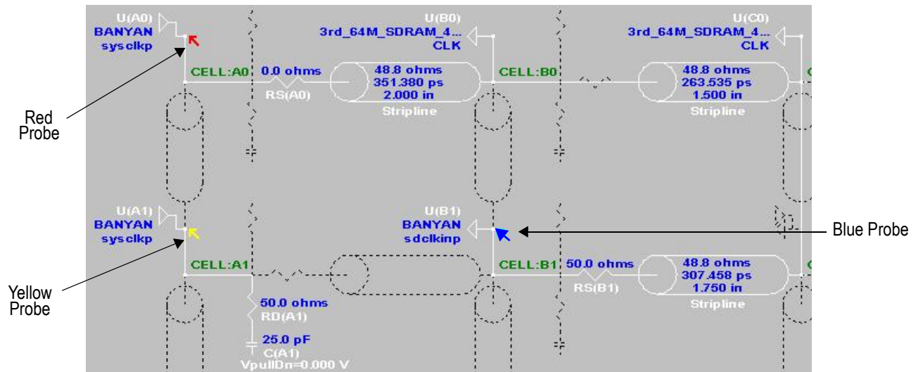
Figure 1 Hyperlynx/Linesim Simulation Circuit
