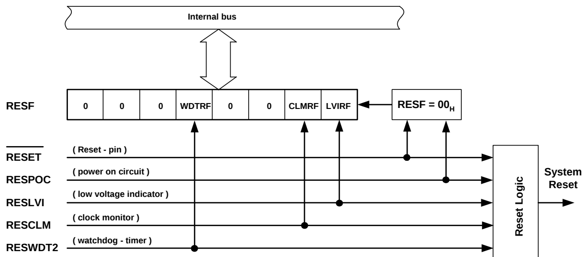
Figure 3-1. Example for a reset control flag register ( RESF )
