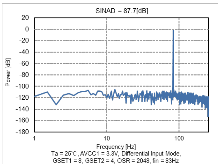
Figure 18. Power versus Frequency (G SET1 = 8, G SET2 = 4, OSR = 2048)
