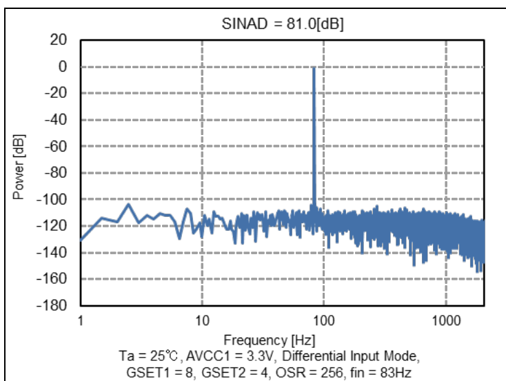
Figure 17. Power versus Frequency (G SET1 = 8, G SET2 = 4, OSR = 256)
