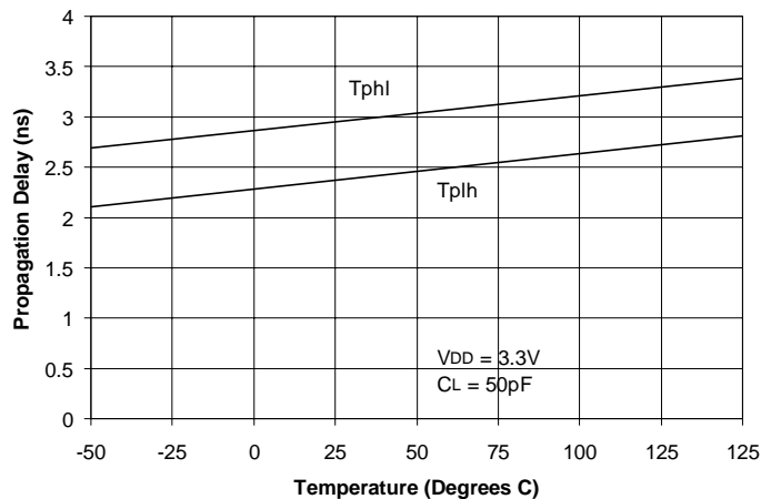
Figure 41, Delay vs. Temperature in an LVC16244
