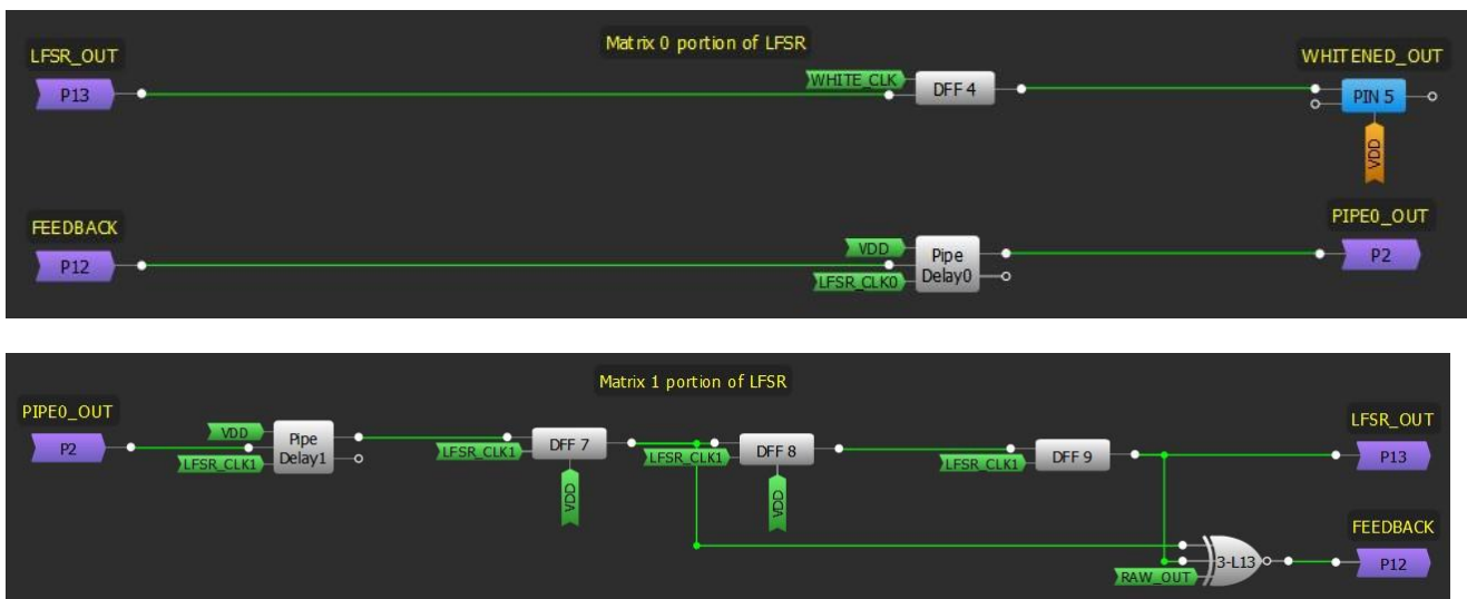
Figure 4. LFSR implementation.
