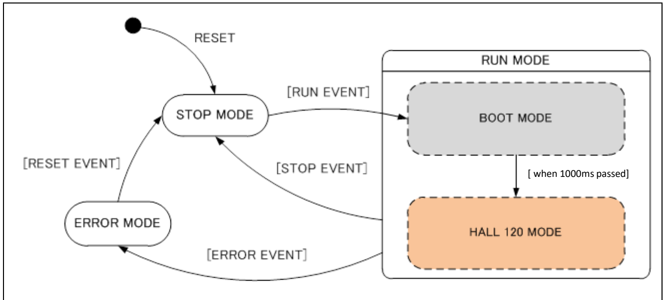
Figure 3-4 状態遷移図
