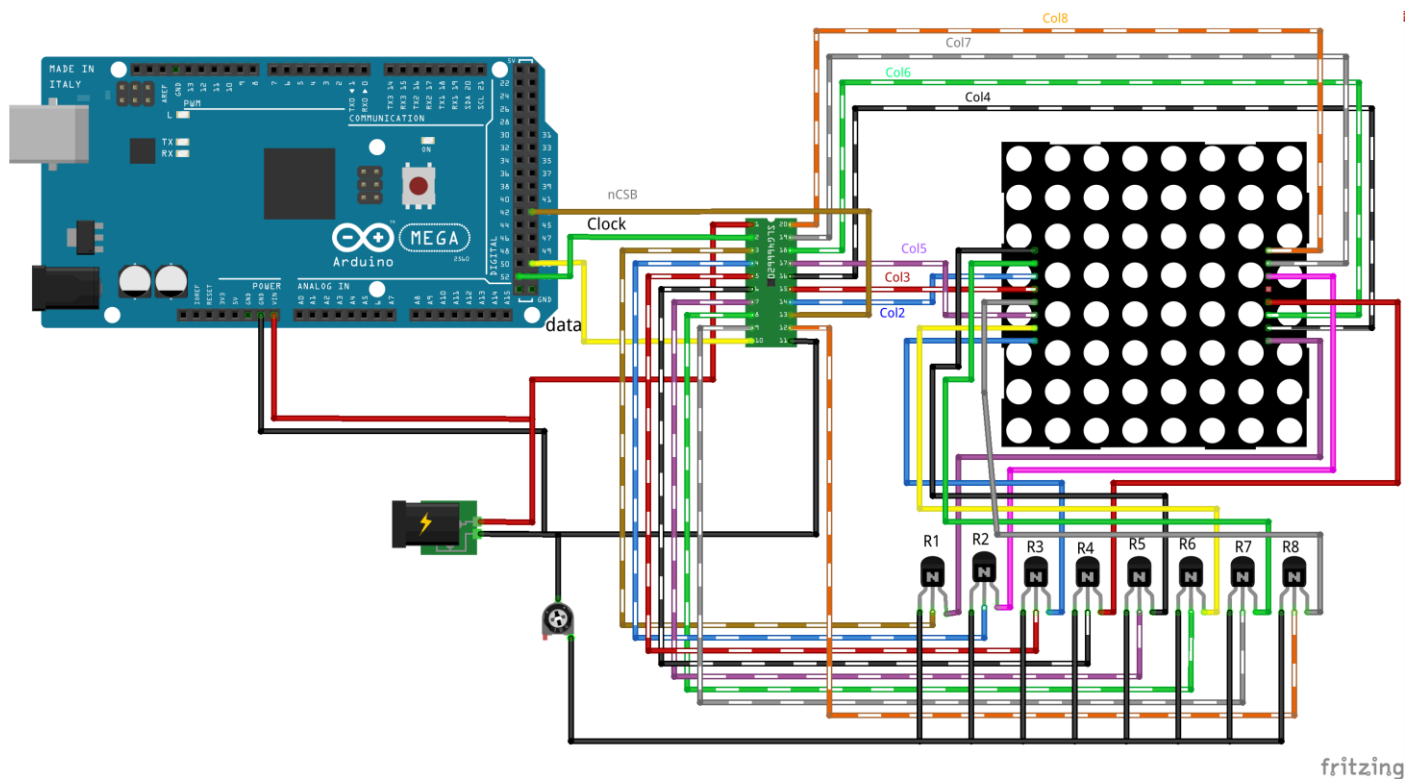
Figure 12. Top-Level Schematic
