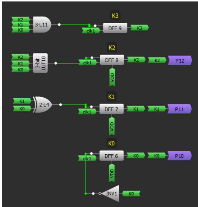
Figure 7. Row counter
