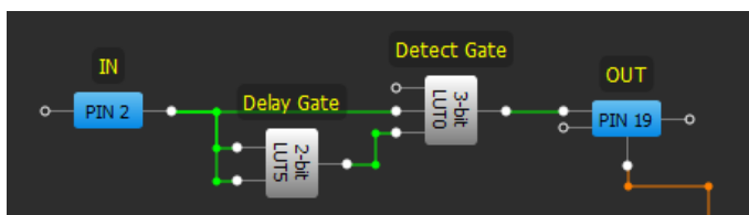
Figure 1. LUT Circuit
