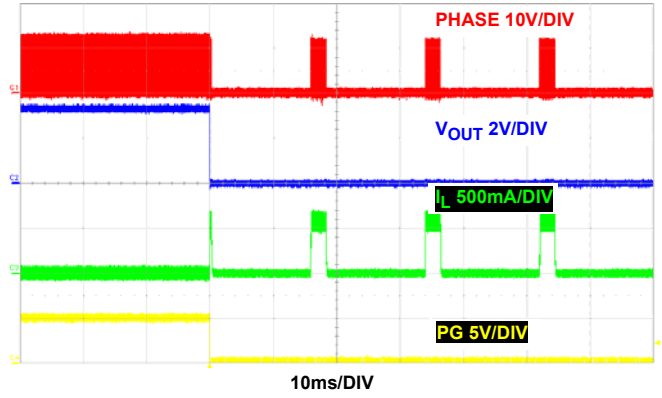
FIGURE 44. OVERCURRENT PROTECTION
