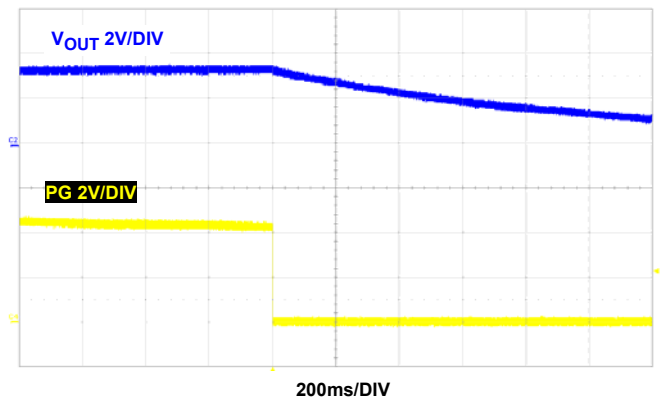
FIGURE 48. OVER-TEMPERATURE PROTECTION
