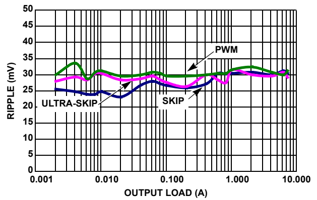
FIGURE 24. V_{OUT1} = 1.5V RIPPLE vs LOAD
