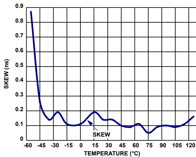
FIGURE 13. DRIVER DIFFERENTIAL SKEW vs TEMPERATURE (ISL3158AE)
