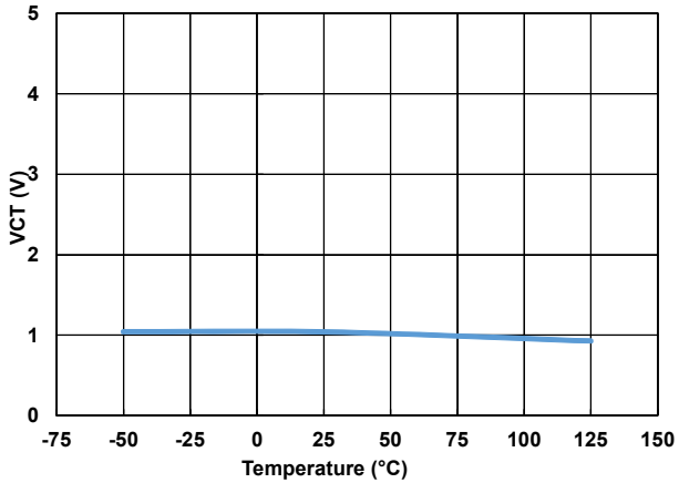
Figure 17. CT Valley Voltage vs Temperature
