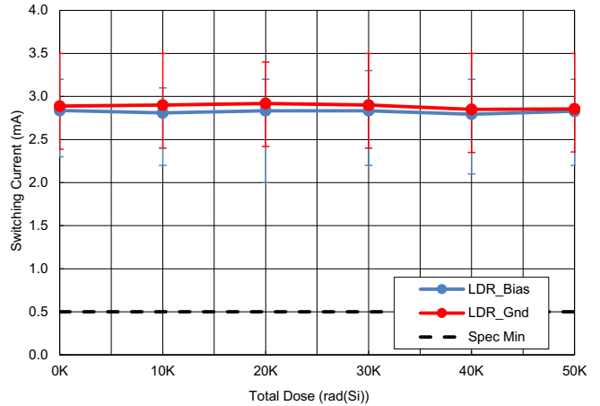
Figure 33. 5V Low-to-High Switching Current vs TID
