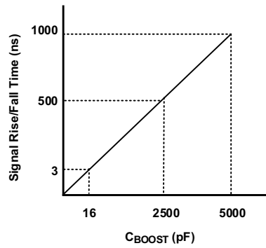
Figure 19. Boost Capacitor (C BOOST ) Selector Guide
