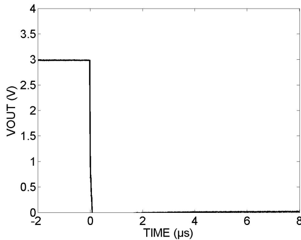
Figure 38. 0mA in Coil, Output Latched Low, V_{DD} = 3.0\text{V}
