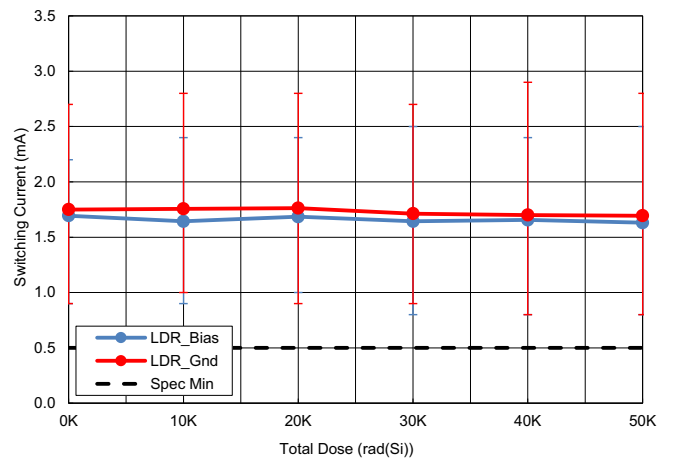
Figure 31. 3V Low-to-High Switching Current vs TID
