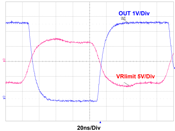
Figure 23. Switching, Coil Current \sim \pm 18mA , C_{BOOST} = 5pF , C_{OUT} = 15pF , V_{DD} = 5V
