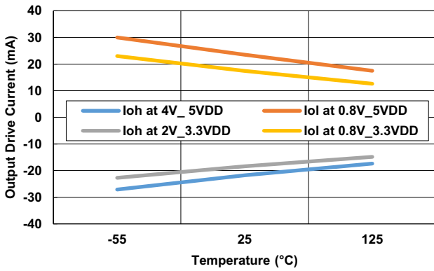
Figure 17. Output Drive Current Capability vs Temperature, Voltage
