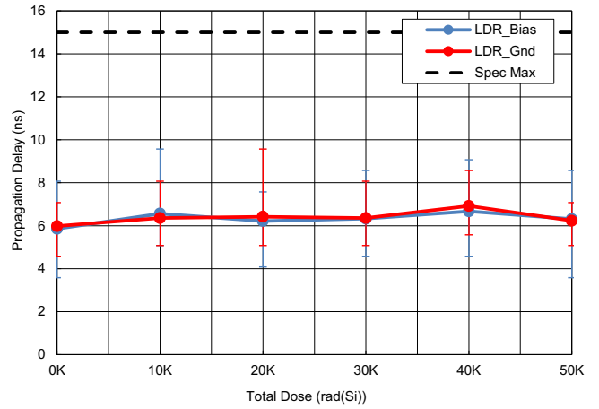
Figure 27. Propagation Delay High-to-Low vs TID
