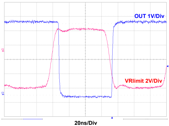
Figure 25. Inverting Configuration, Switching, Coil Current \sim \pm 10mA , C_{BOOST} = 5pF , C_{OUT} = 15pF , V_{DD} = 5V
