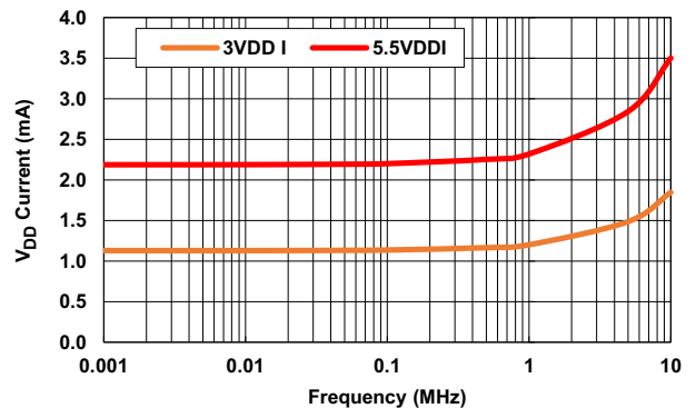
Figure 10. V_{DD} Current vs Frequency, Voltage, 0 load, 50% Duty Cycle
