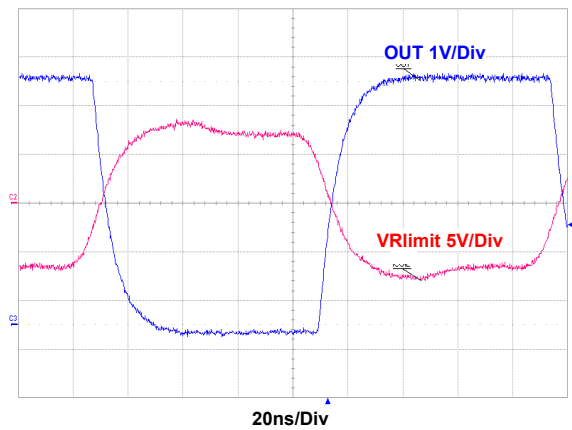
Figure 21. Switching, Coil Current \sim \pm 18mA , C_{BOOST} = 15pF , C_{OUT} = 15pF , V_{DD} = 5V
