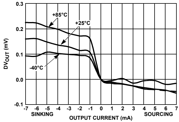
FIGURE 36. LOAD REGULATION
