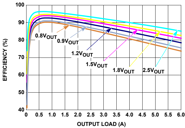
FIGURE 8. EFFICIENCY vs LOAD (2MHz 3.3V V_{IN} PWM)
