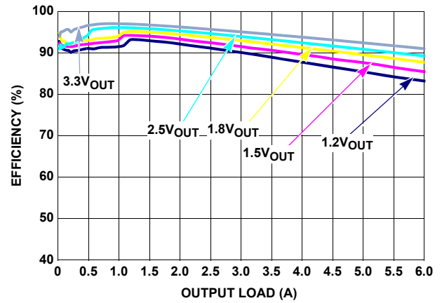
FIGURE 7. EFFICIENCY vs LOAD (1MHz 5V V_{IN} PFM)
