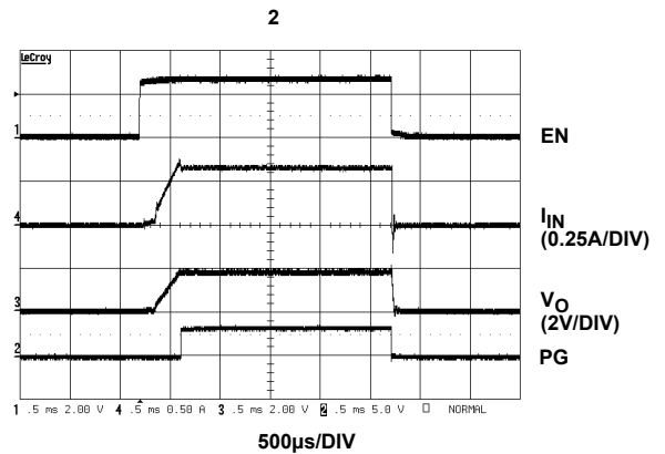
FIGURE 11. ENABLE AND SHUT-DOWN
