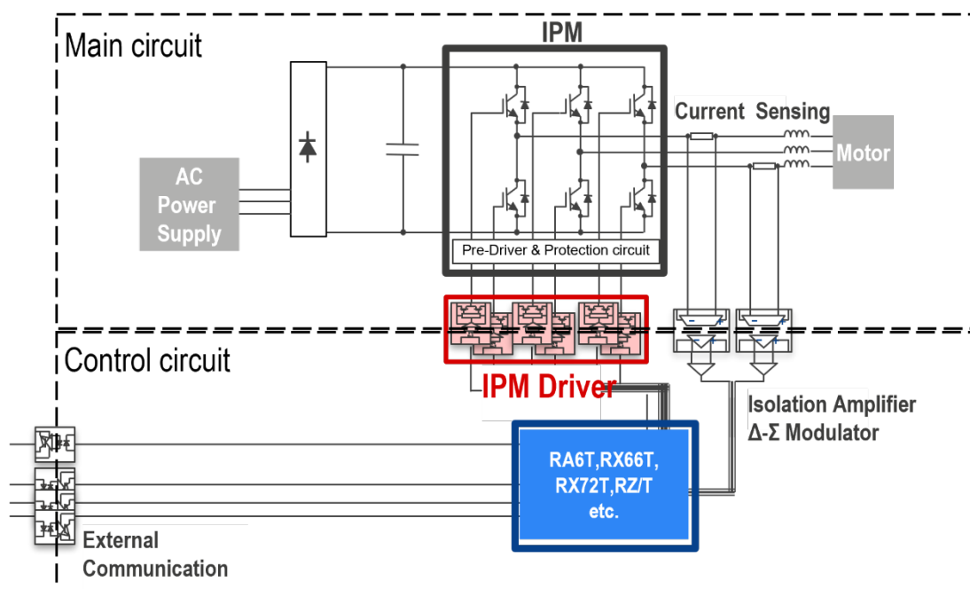
Figure 1. Inverter Circuit of the General-purpose Inverter
