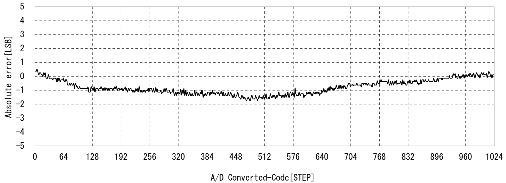
R32C/116, 117, 118 Group A/D Accuracy (Vcc=Avcc=Vref=5V, Ta=25°C, \phi_{AD} =16MHz, Resolution=10bits, with sample and hold function)
