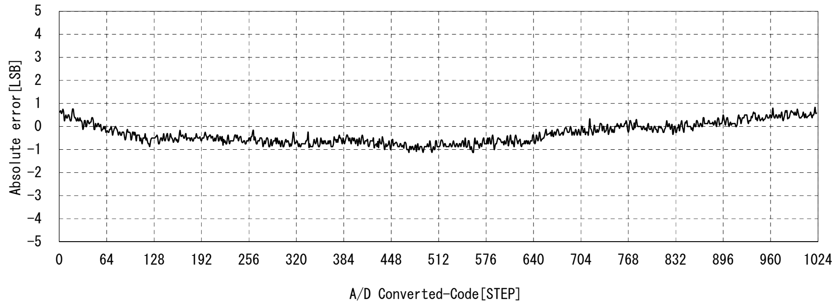
R32C/116, 117, 118 Group A/D Accuracy (Vcc=Avcc=Vref=3.3V, Ta=25°C, \phi AD=10MHz, Resolution=10bits, with sample and hold function)
