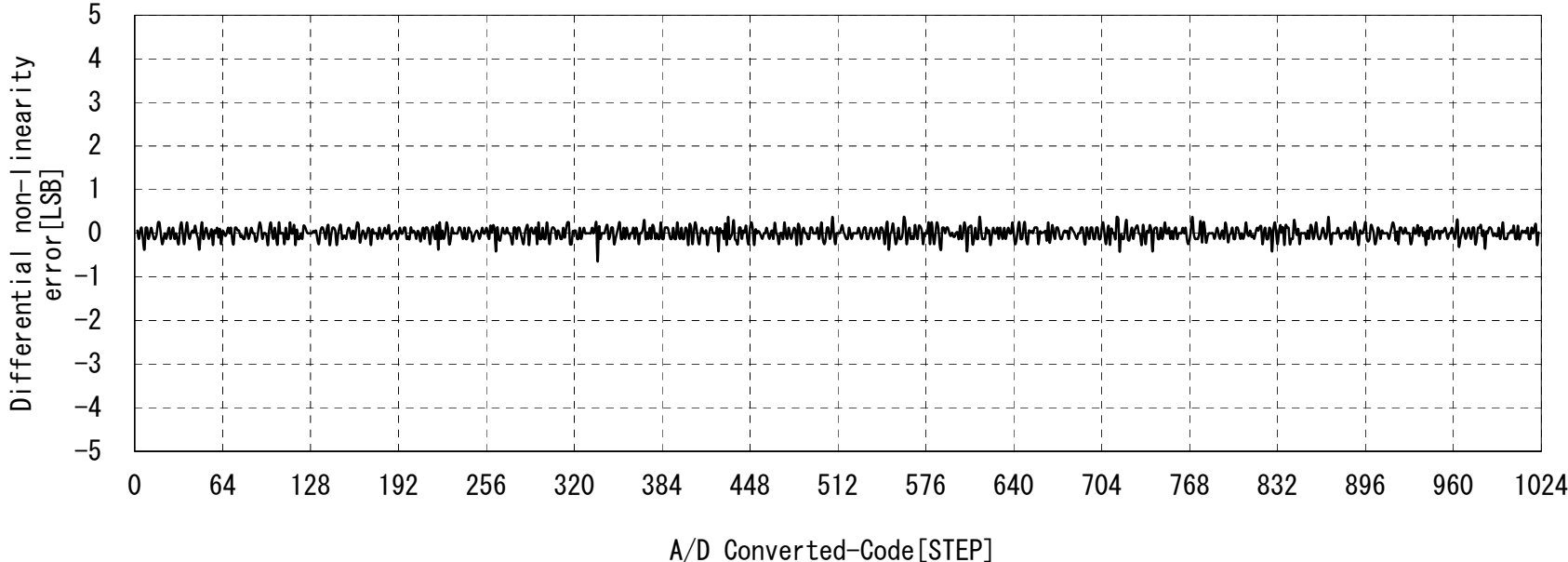
R32C/116, 117, 118 Group A/D Accuracy (Vcc=Avcc=Vref=3.3V, Ta=25°C, \phi AD=10MHz, Resolution=10bits, with sample and hold function)
