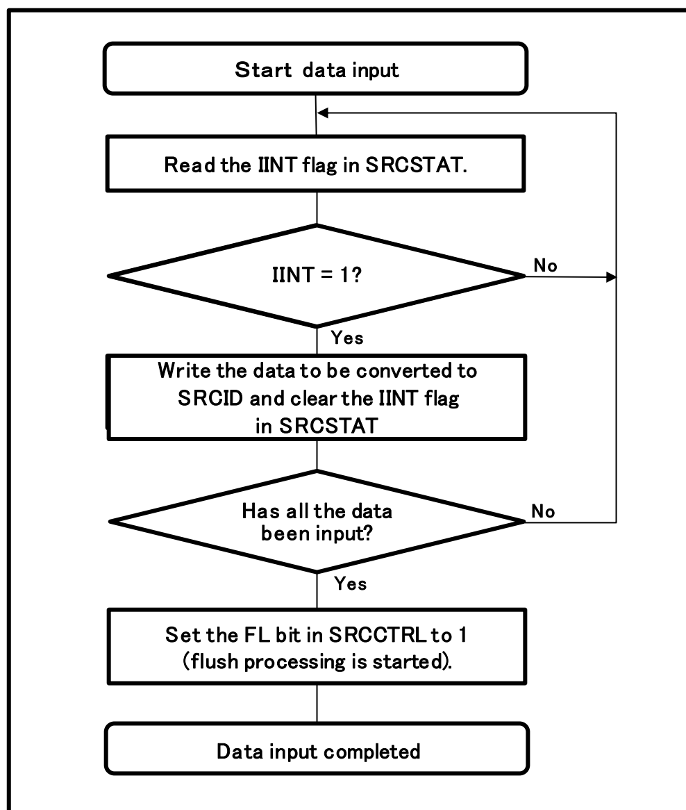
Figure 48.3 Flowchart for Data Input
