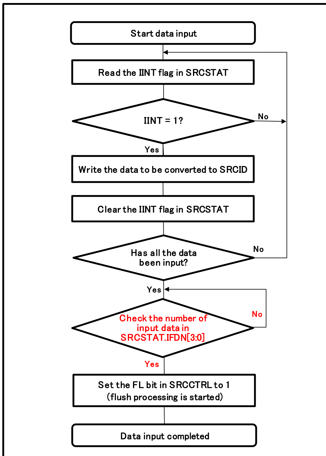
Figure 48.3 Flowchart for Data Input
