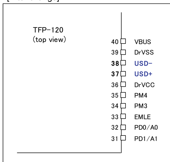
Figure 1.2 Pin Assignments
