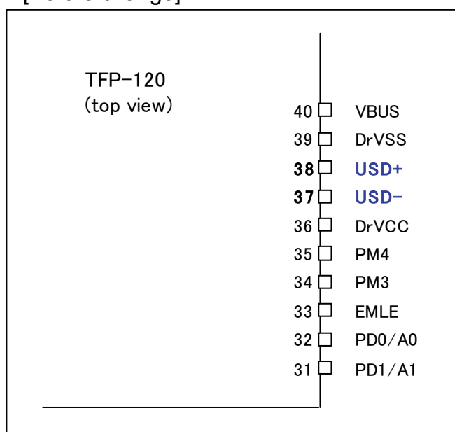
Figure 1.2 Pin Assignments
