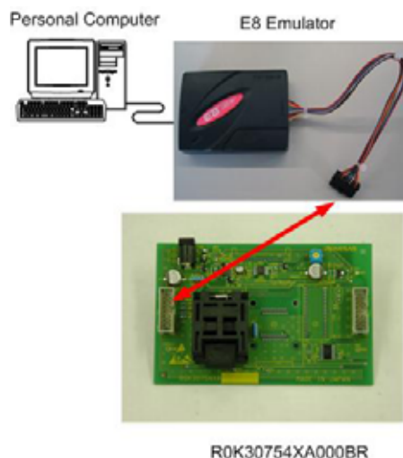
Figure 7.1 Connecting Example 1
