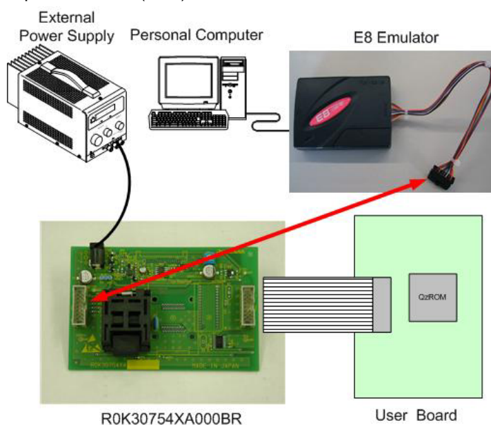
Figure 7.2 Connecting Example 2
