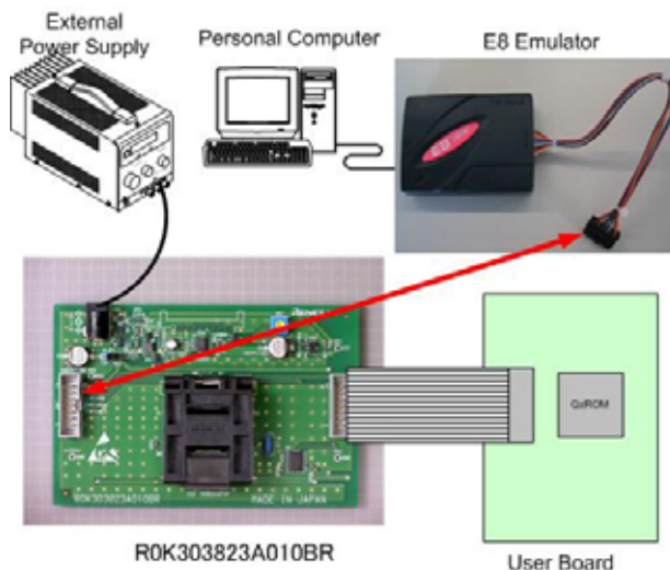
Figure 7.2 Connecting Example 2
