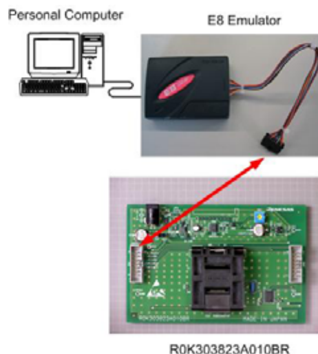
Figure 7.1 Connecting Example 1
