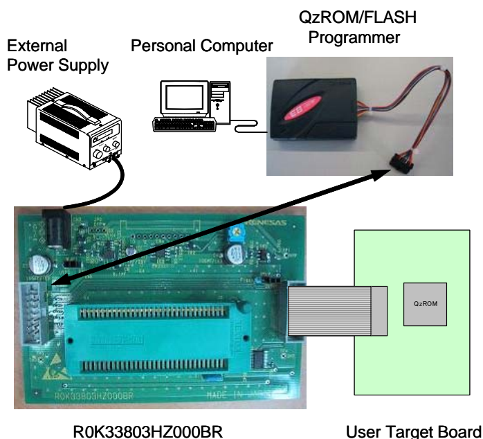
Figure 7.2 Connecting Example 2
