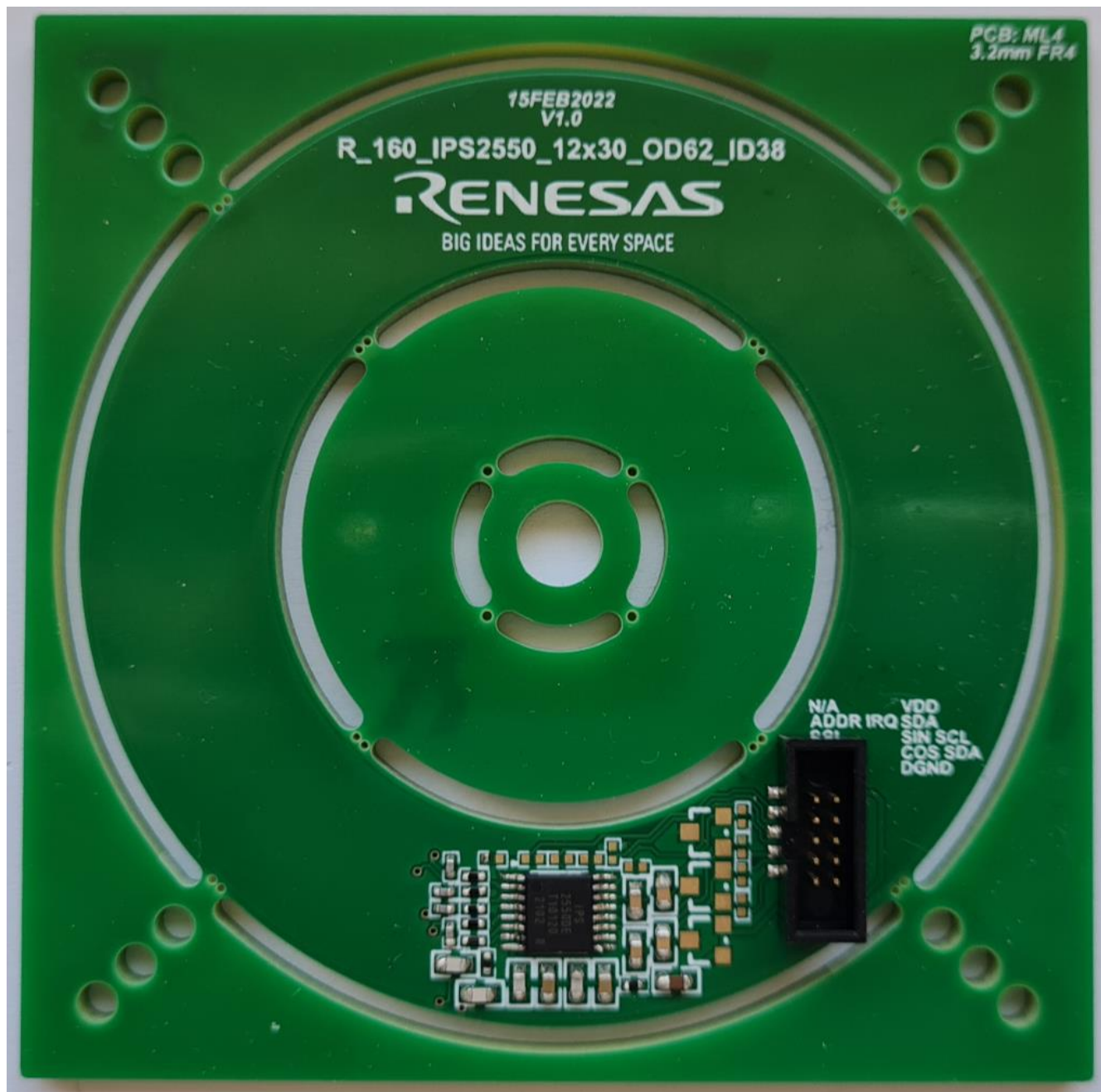
Figure 1. Sensor Board
