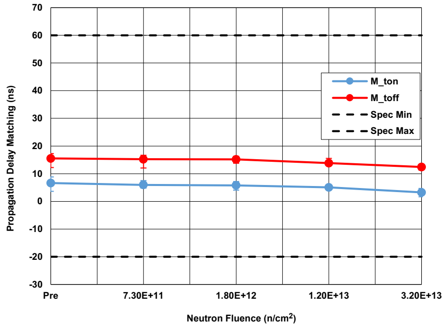
Figure 17. IS-2100ARH turn-on propagation delay matching (M_ton) following neutron irradiation to each level. The error bars represent the minimum and maximum measured values. The SMD limits are -20ns minimum and 60ns maximum.
