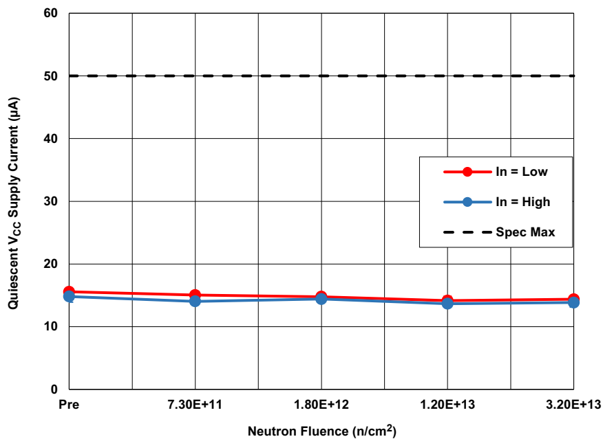
Figure 2. IS-2100ARH quiescent V CC supply current (I QCC ) with inputs low or high following neutron irradiation to each level. The error bars represent the minimum and maximum measured values. The SMD limit is 50µA maximum.
