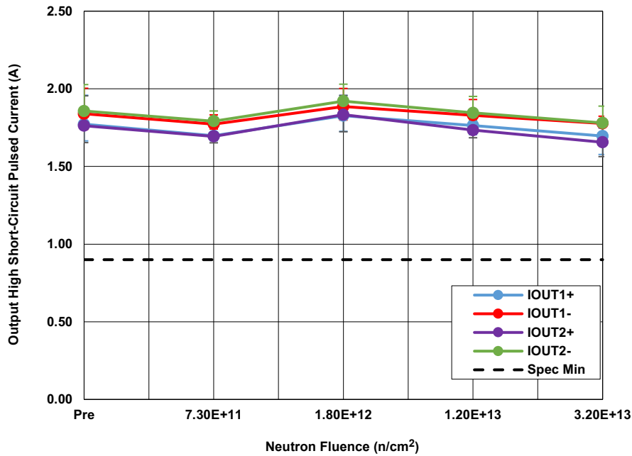
Figure 9. IS-2100ARH output high short-circuit current (pulsed) (+I O UT , -I O UT ) following neutron irradiation to each level. The error bars represent the minimum and maximum measured values. The SMD limit is 0.9A minimum.
