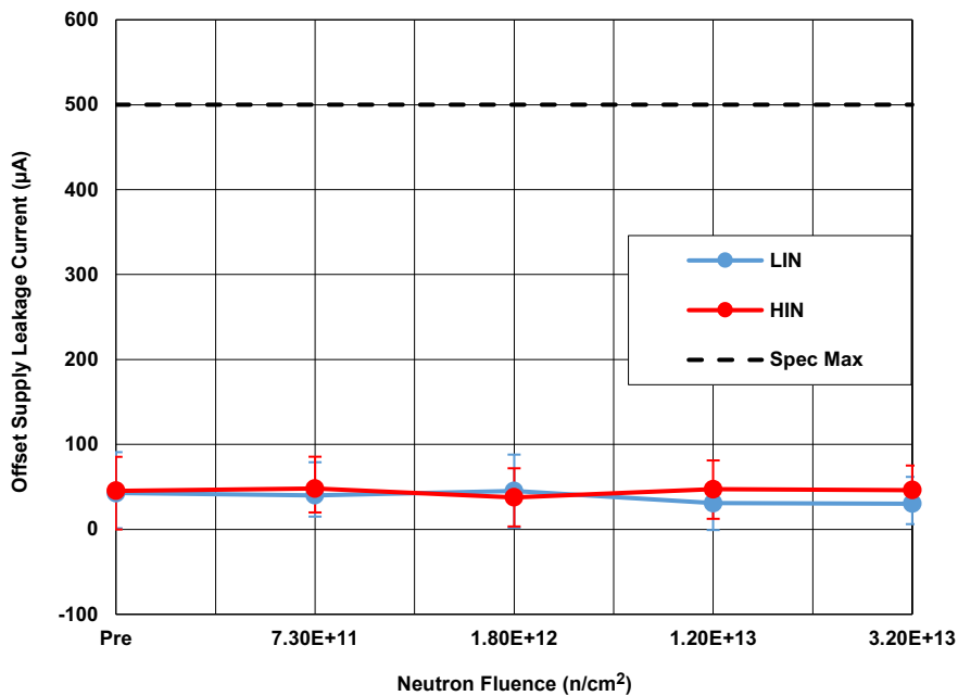
Figure 4. IS-2100ARH offset supply leakage current ( I_{LK} ) following neutron irradiation to each level. The error bars represent the minimum and maximum measured values. The SMD limit is 500\mu A maximum.
