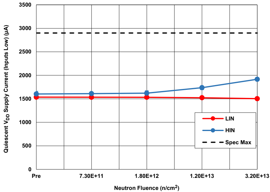
Figure 1. IS-2100ARH quiescent V DD supply current (I QDD ) with inputs low (L IN and H IN ) following neutron irradiation to each level. The error bars represent the minimum and maximum measured values. The SMD limit is 2900µA maximum.
