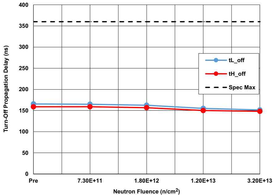
Figure 11. IS-2100ARH high-side and low-side turn-off propagation delay (tL_off, tH_off) following neutron irradiation to each level. The error bars represent the minimum and maximum measured values. The SMD limit is 360ns maximum.
