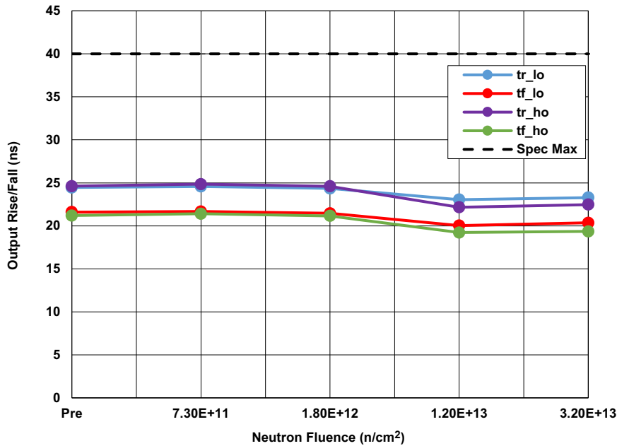
Figure 14. IS-2100ARH output rise and fall times (t R , t F ) following neutron irradiation to each level. The error bars represent the minimum and maximum measured values. The SMD limit is 40ns maximum.
