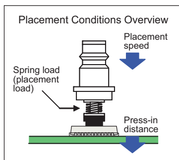
Figure 4.1 Placement Conditions
