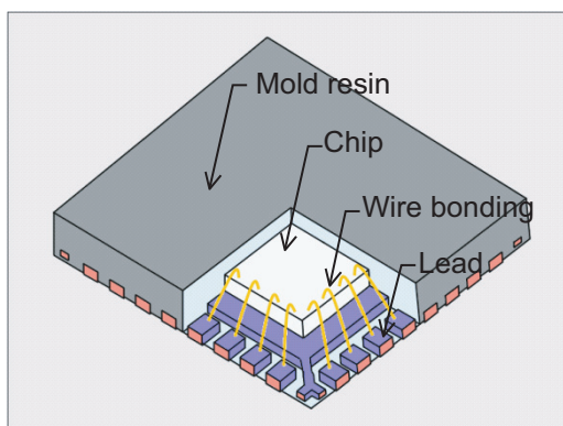
Figure 1.7 Basic Structure
