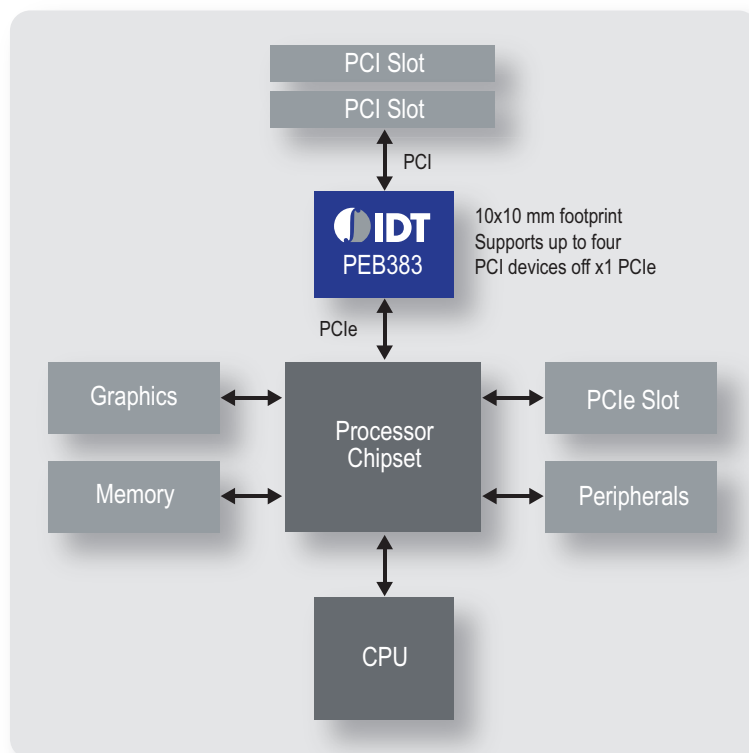
Figure 1 Motherboard Application
