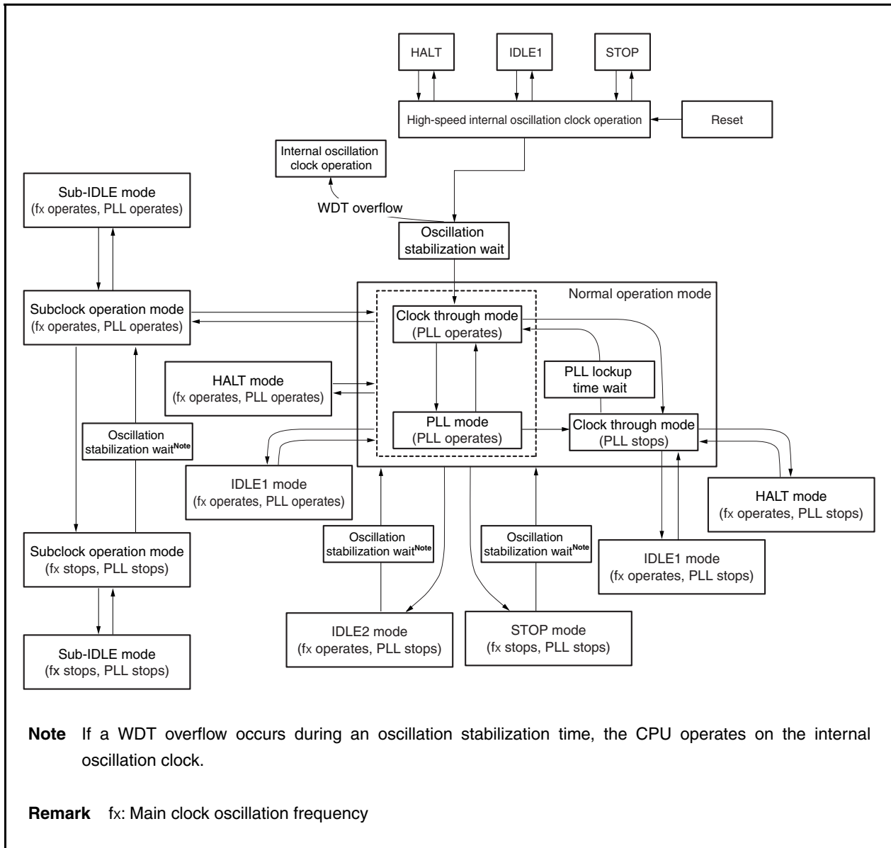
Figure 20-1. Status Transition
