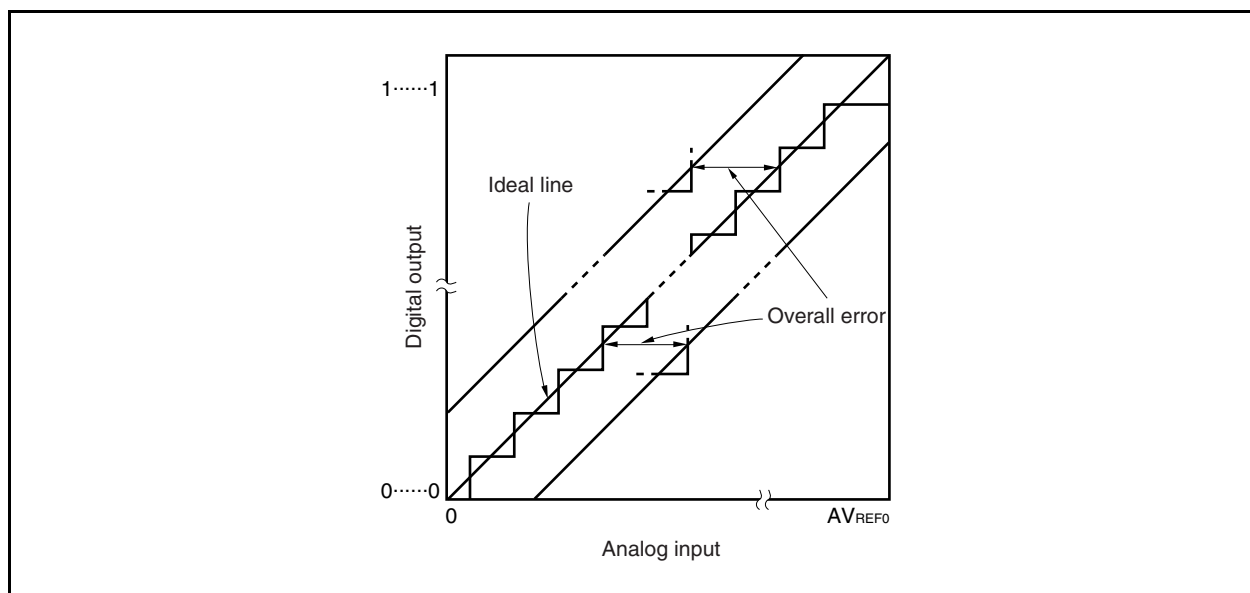
Figure 13-15. Overall Error
