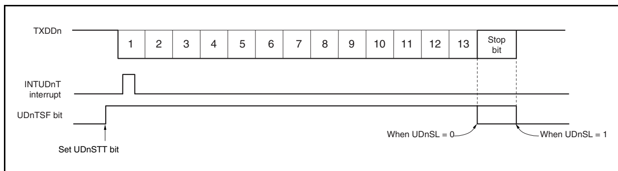
Figure 14-8. SBF Transmission
