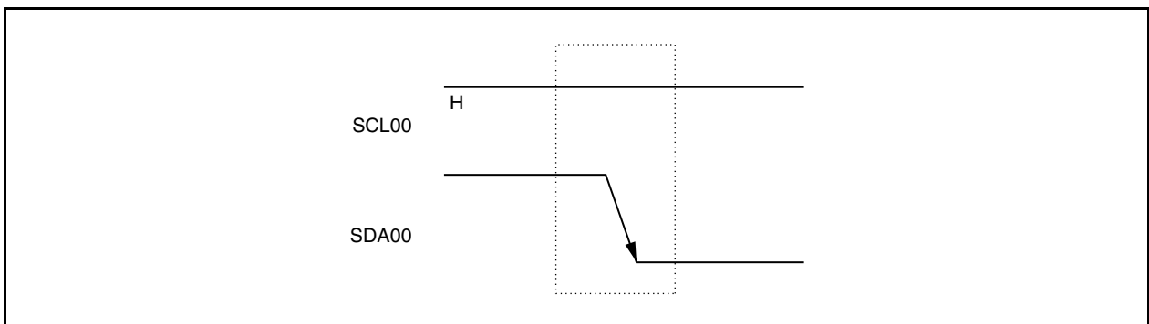
Figure 16-6. Start Conditions
