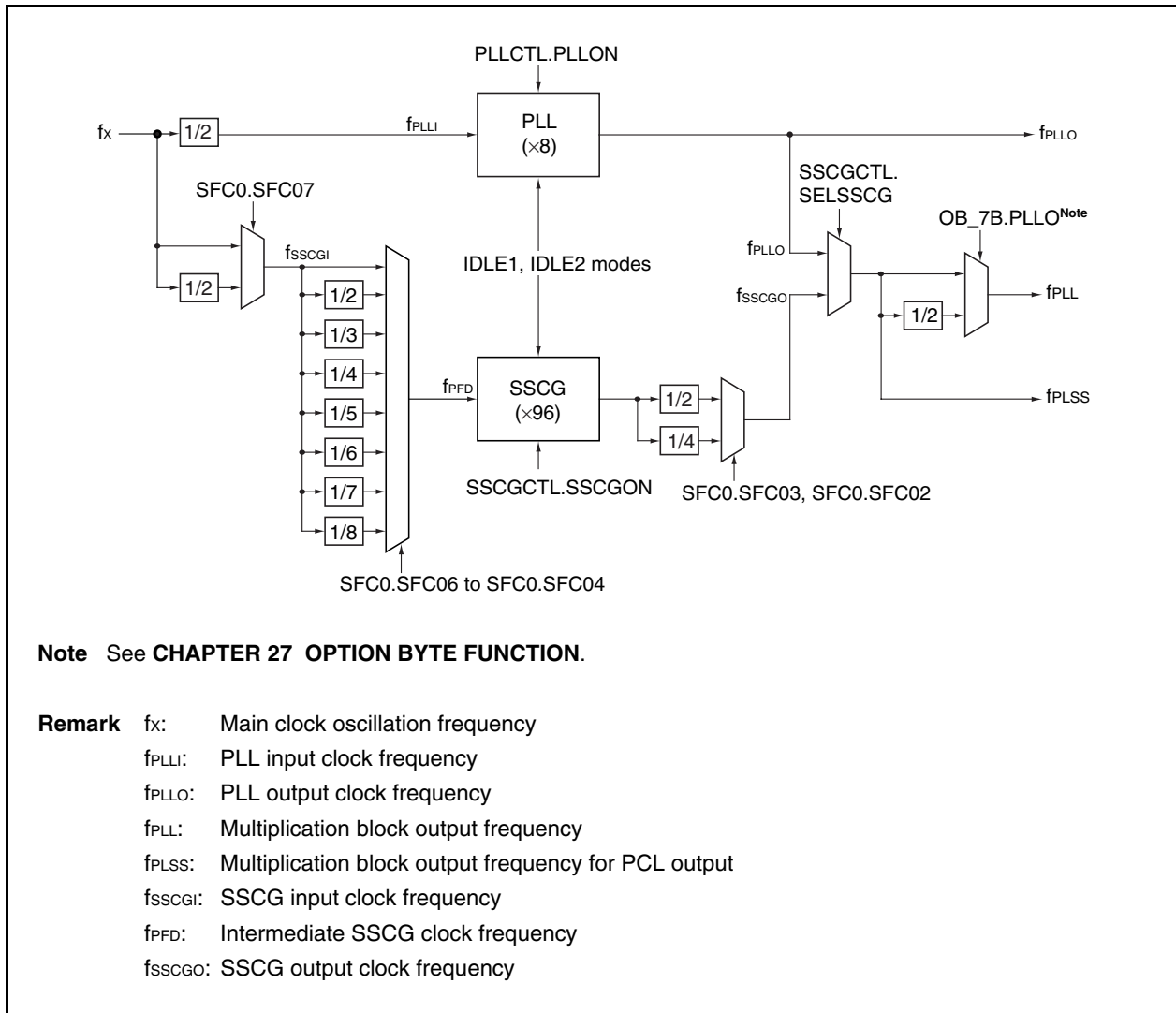
Figure 6-2. PLL/SSCG Circuit
