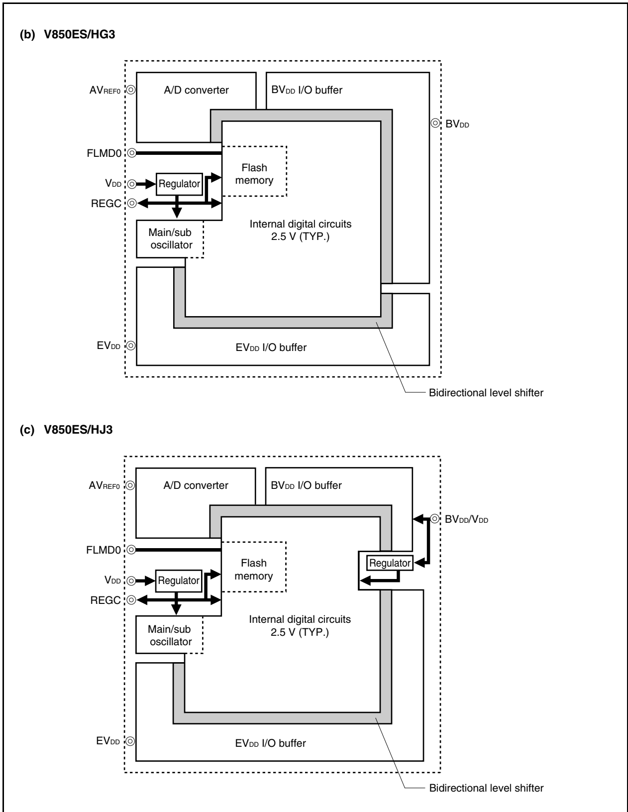
Figure 25-1. Regulator (2/2)
