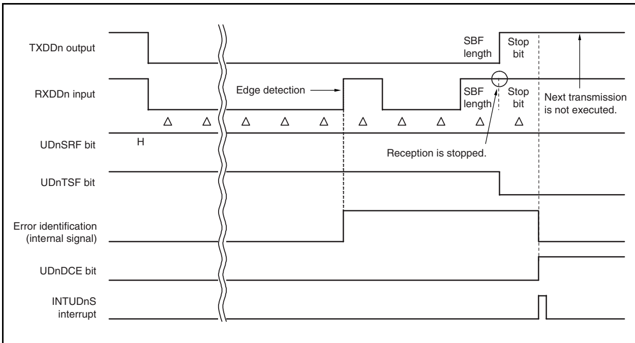
Figure 14-15. Timing Example of Consistency Error Occurrence During SBF Transmission When UDnSRF = 1 (if Reception Is in Progress When Transmission of Stop Bit Is Started (Data Input Immediately Before Is “0”))
