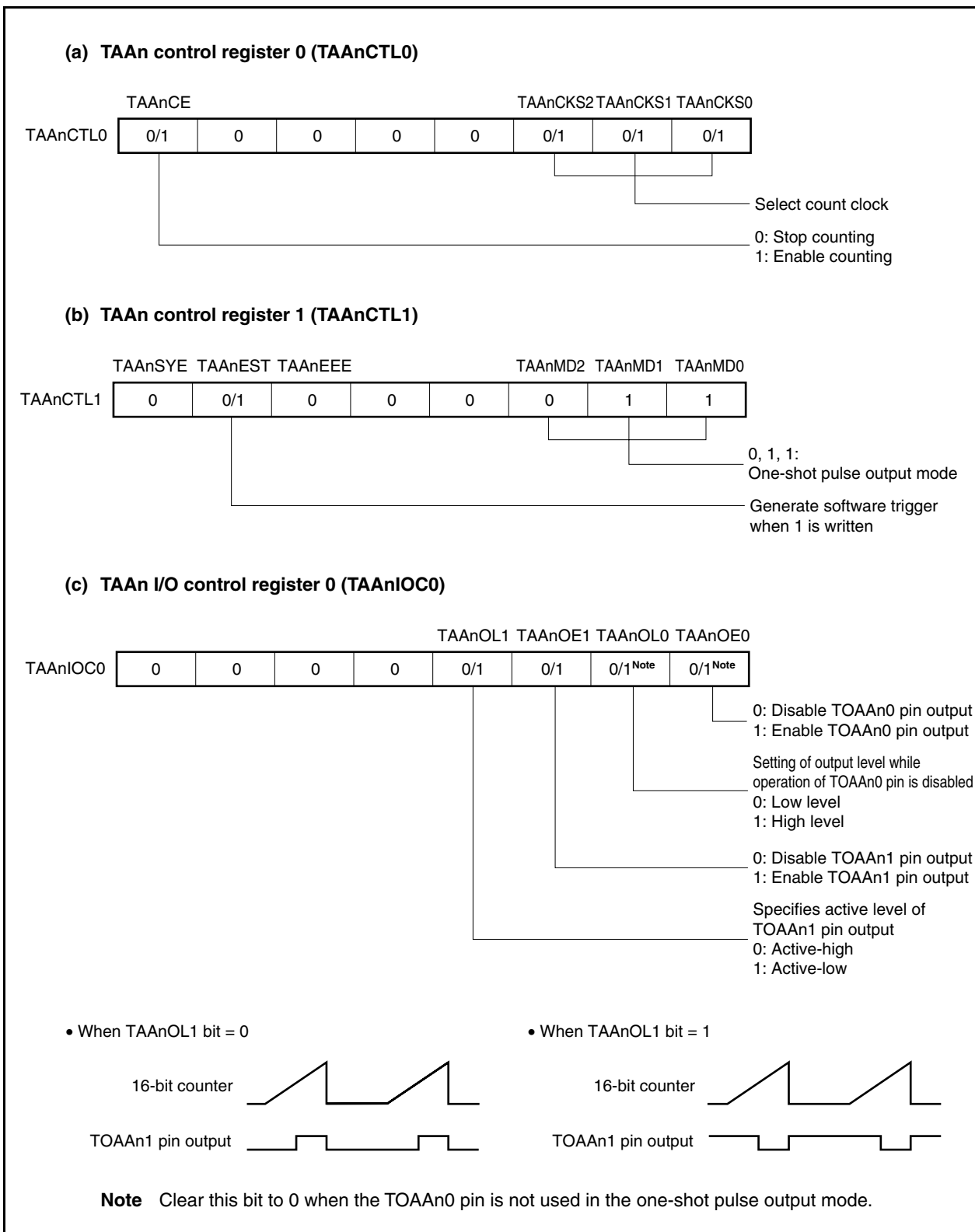
Figure 7-22. Register Setting for Operation in One-Shot Pulse Output Mode (1/2)
