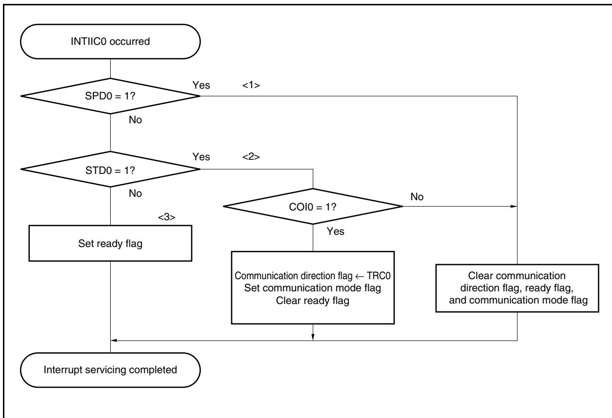
Figure 16-20. Slave Operation Flowchart (2)
