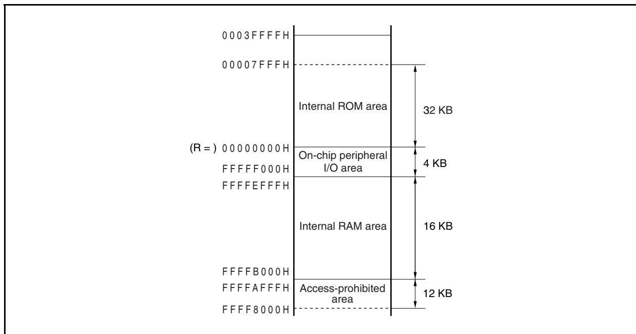
Figure 3-11. Wraparound ( \mu PD70F3755)
