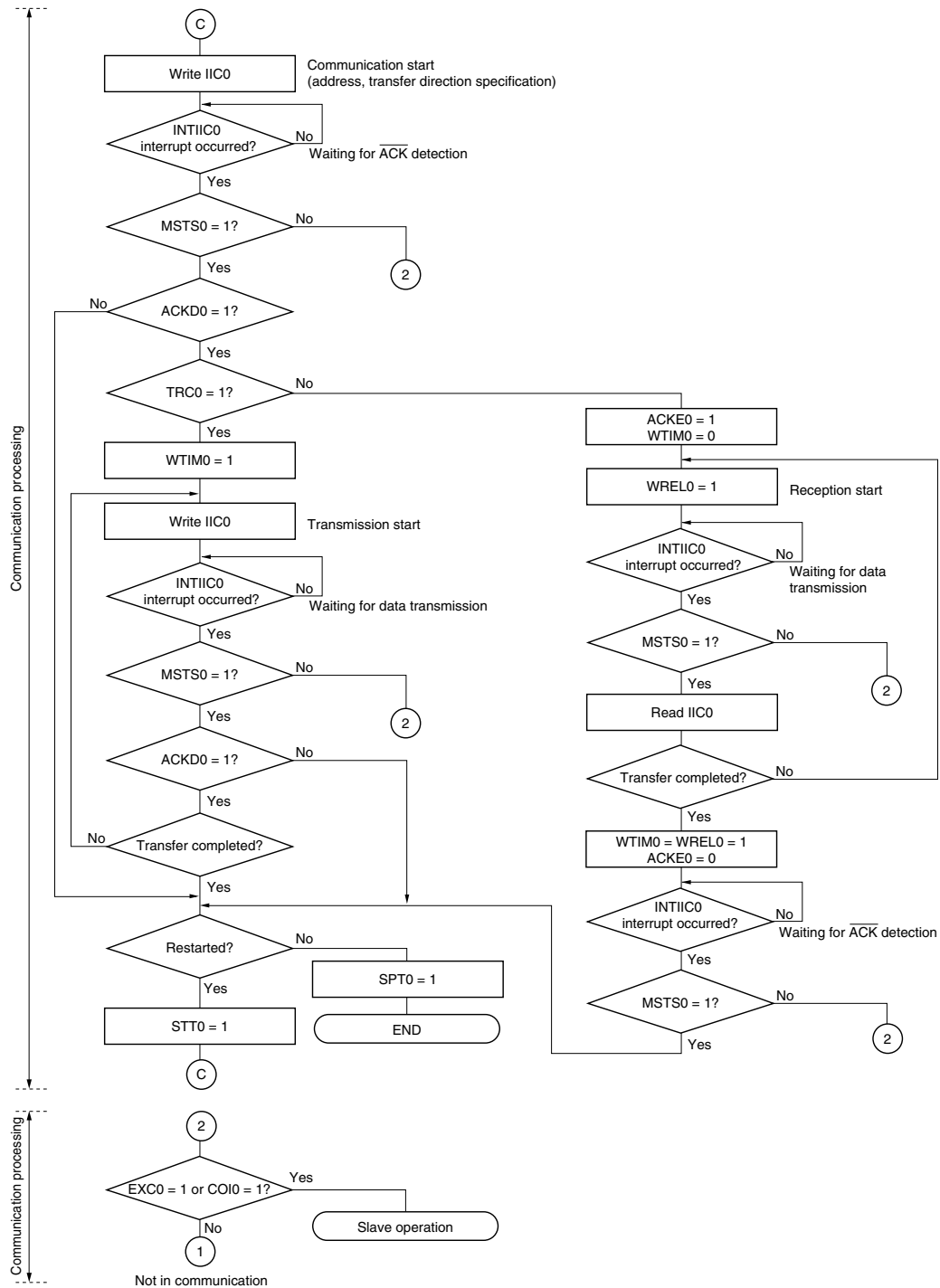
Figure 16-17. Master Operation in Multimaster System (3/3)
