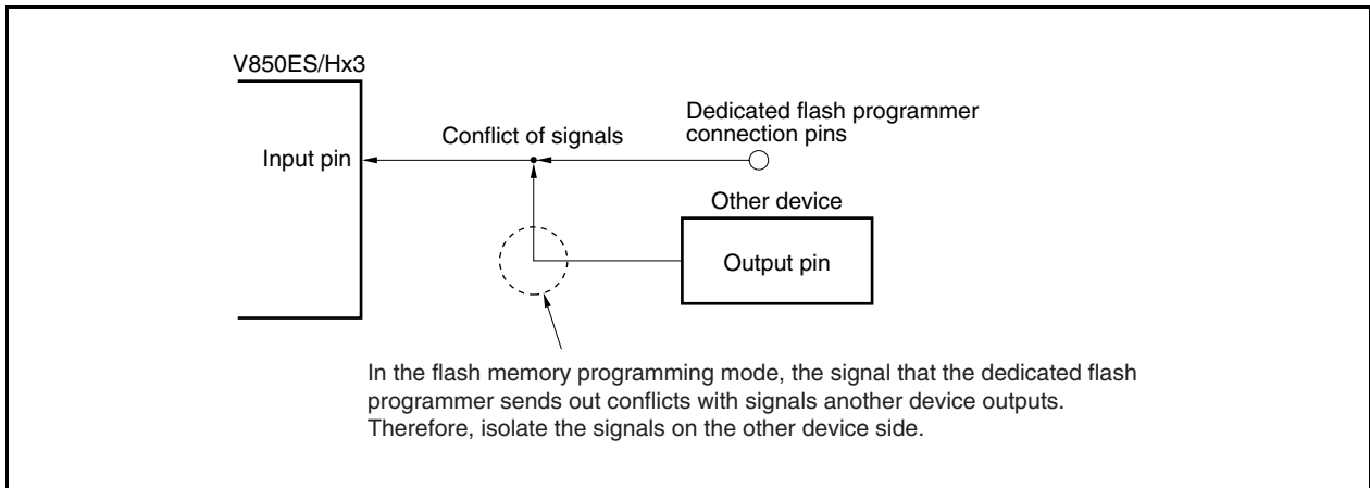
Figure 26-15. Conflict of Signals (Serial Interface Input Pin)
