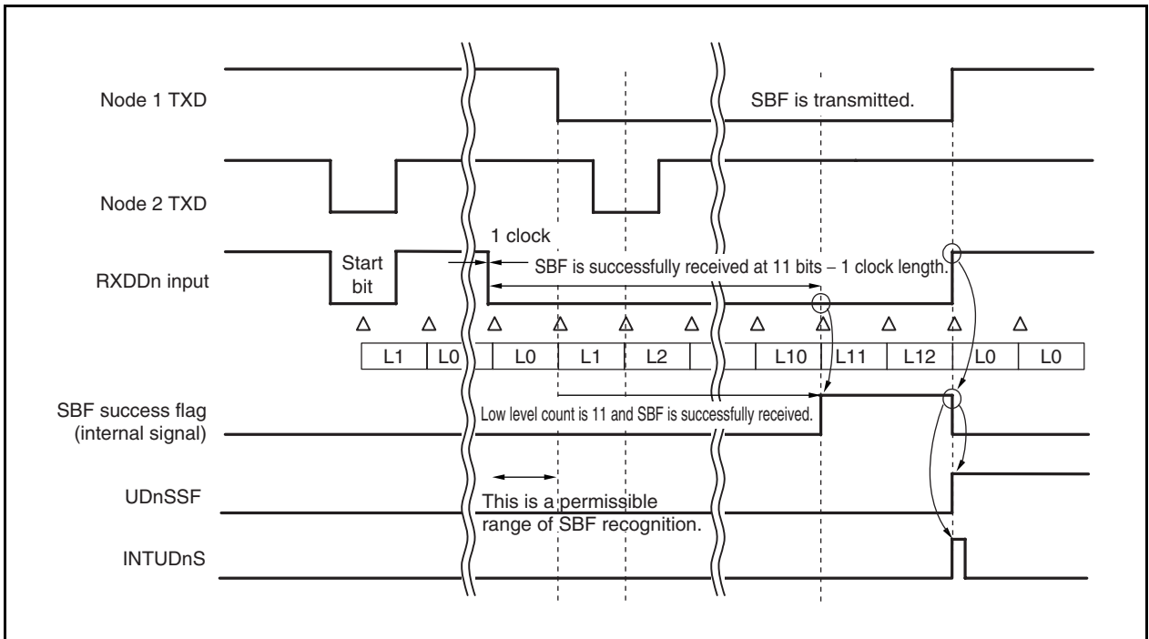
Figure 14-24. Example of Successful Reception of SBF with the Longest Width
