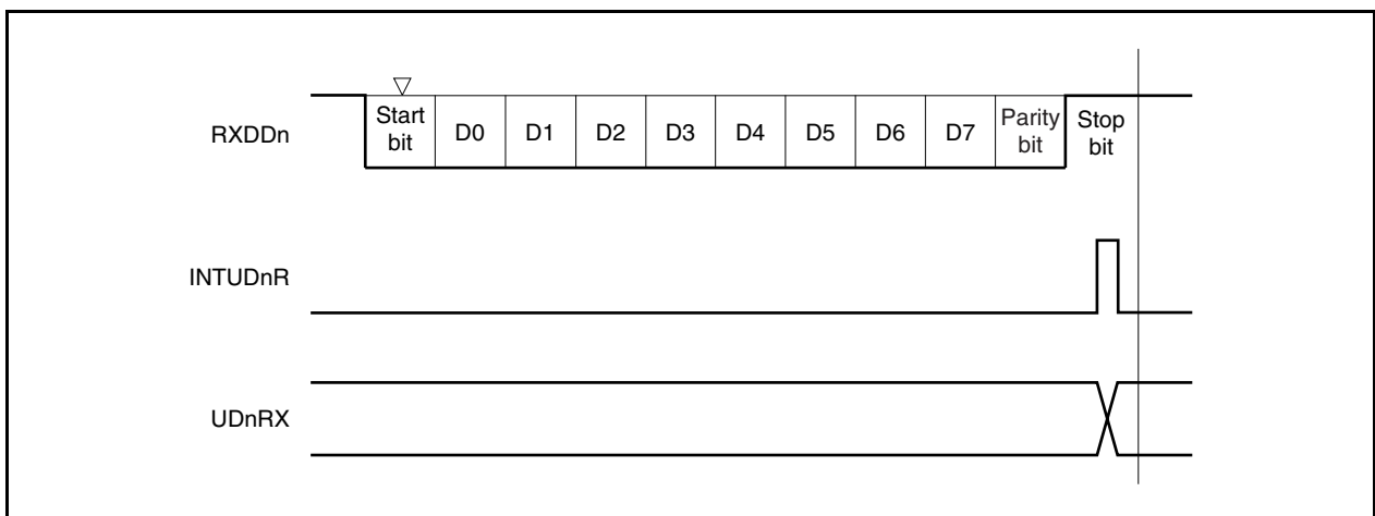
Figure 14-28. UART Reception
