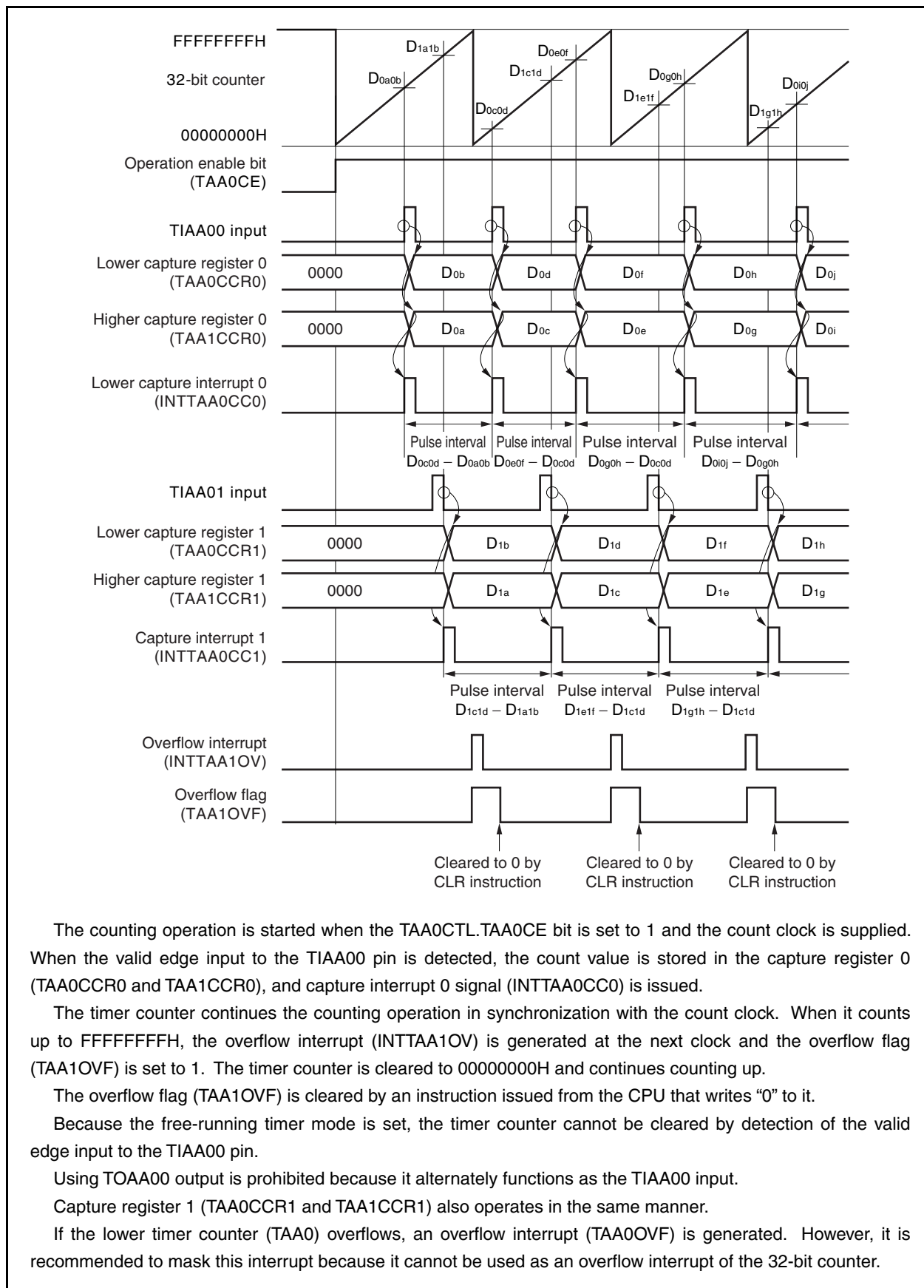
Figure 7-46. Example of Basic Timing When TAA0 and TAA1 Are Connected in Cascade
