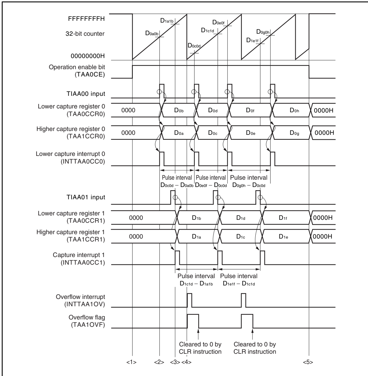
Figure 7-45. Operation Flow in Cascade Connection (1/2)
