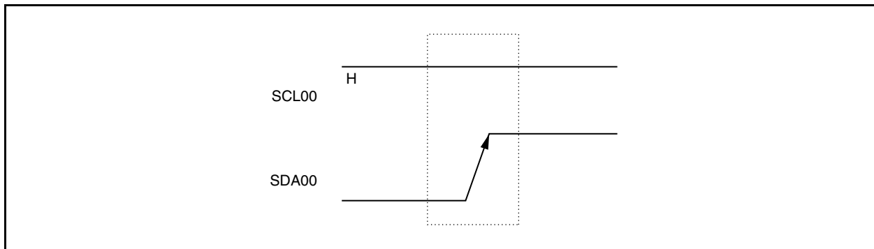
Figure 16-10. Stop Condition
