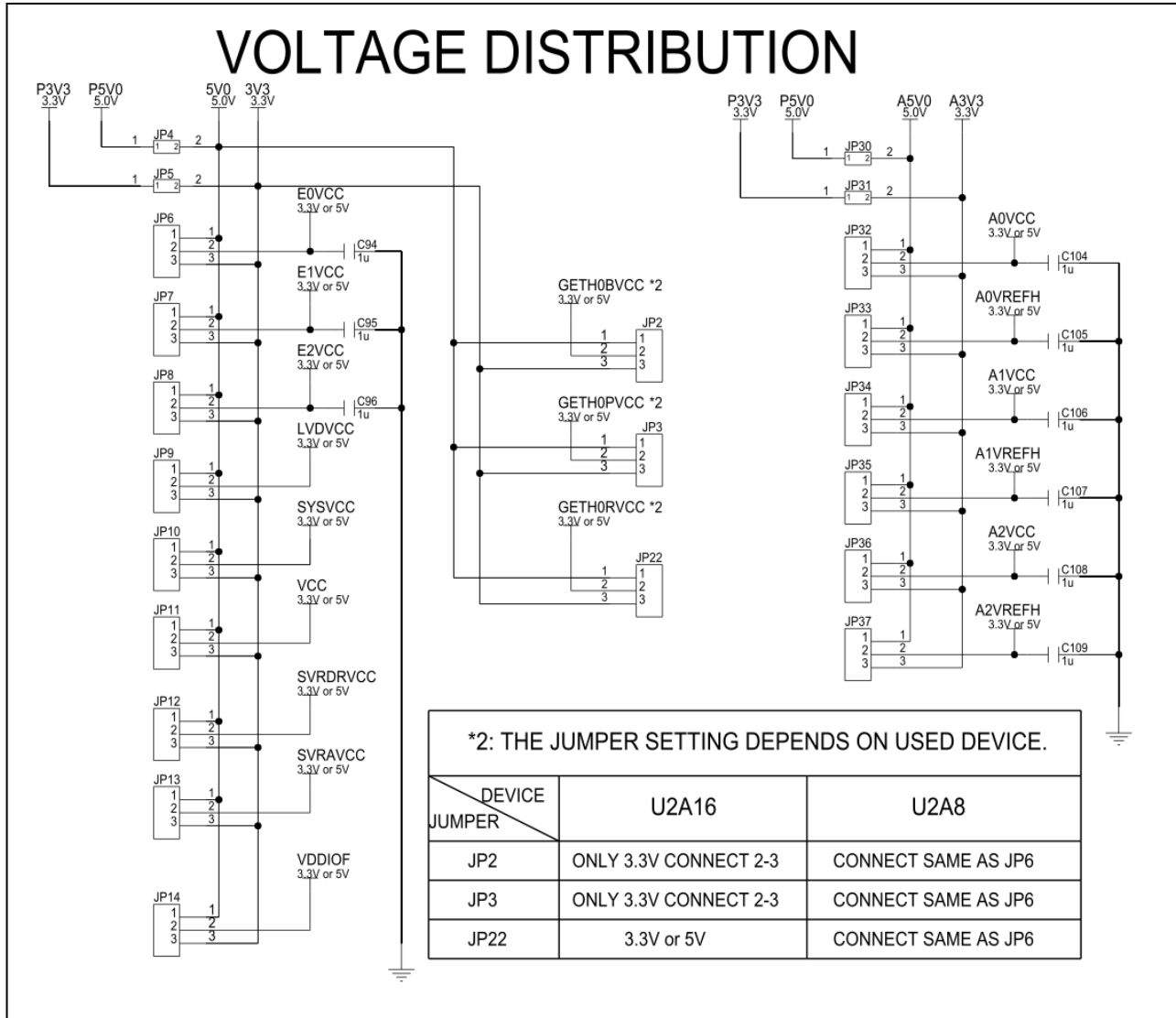
Figure 3.1 Voltage distribution
