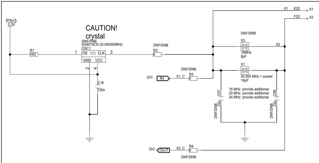
Figure 4.1 Clock supply
