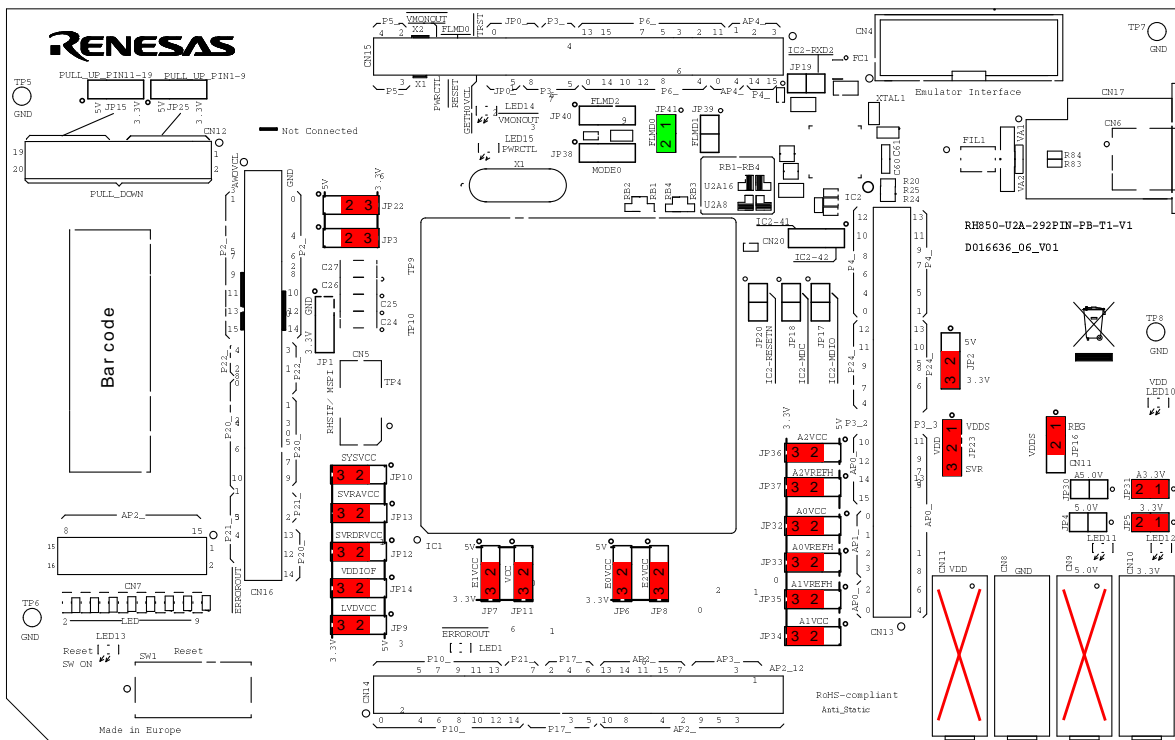
Figure 8.1 Stand-alone operation with minimum external power supply
