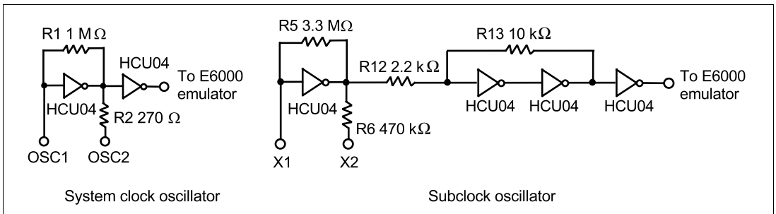
Figure 7 System Clock Oscillator Circuit
