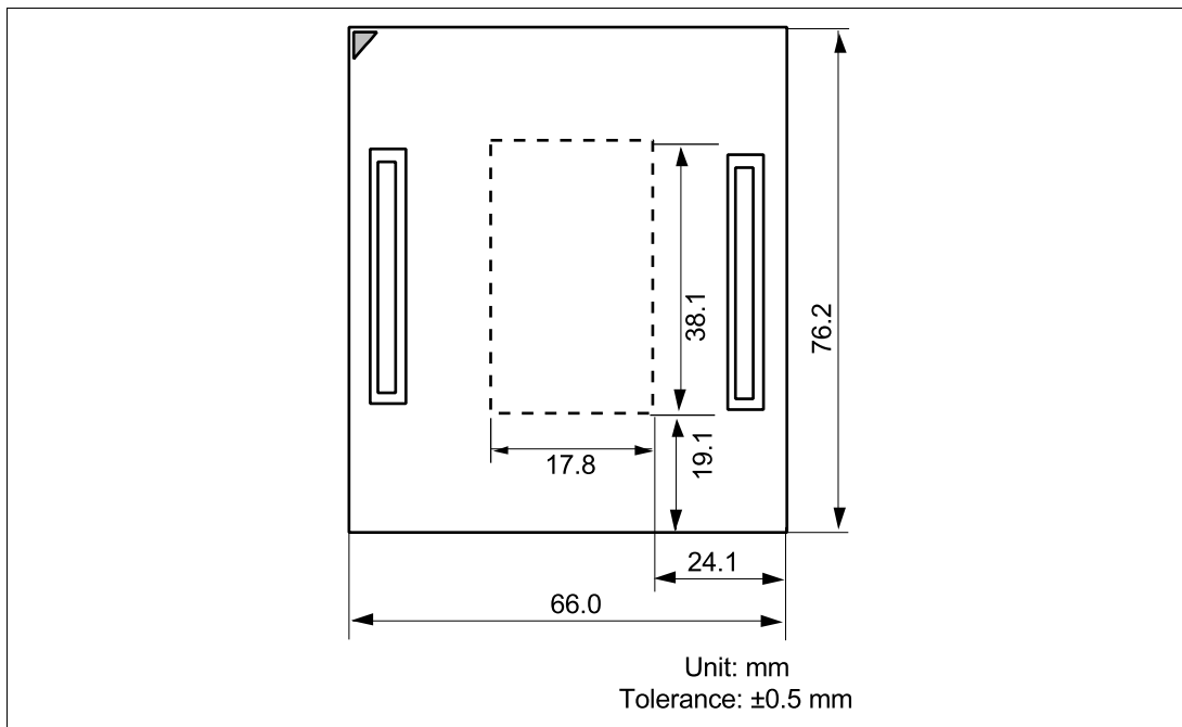
Figure 5 Dimensions for User System Interface Cable Head
