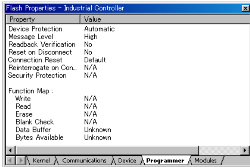
図 8-11 Programmer Properties
