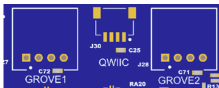
Figure 12. Seeded Grove ® and SparkFun Qwiic ® Connector Footprints
