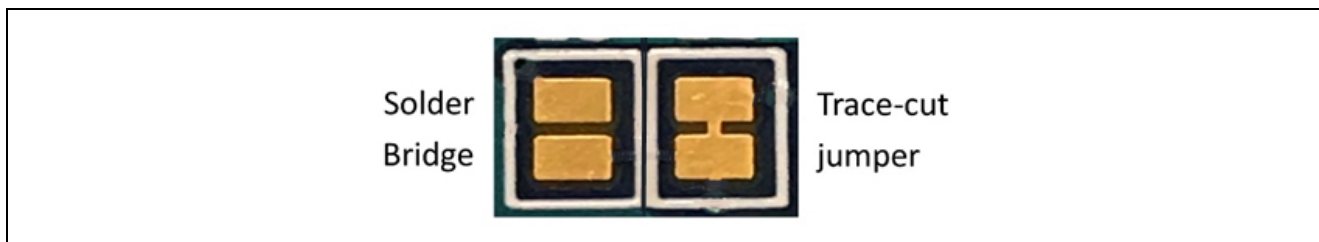
Figure 6. Copper Jumpers
