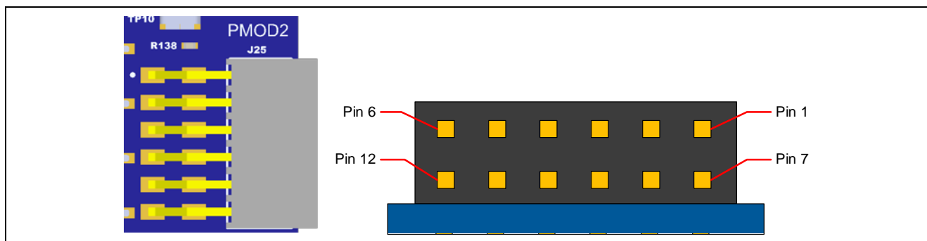
Figure 14. Pmod 2 Connector
