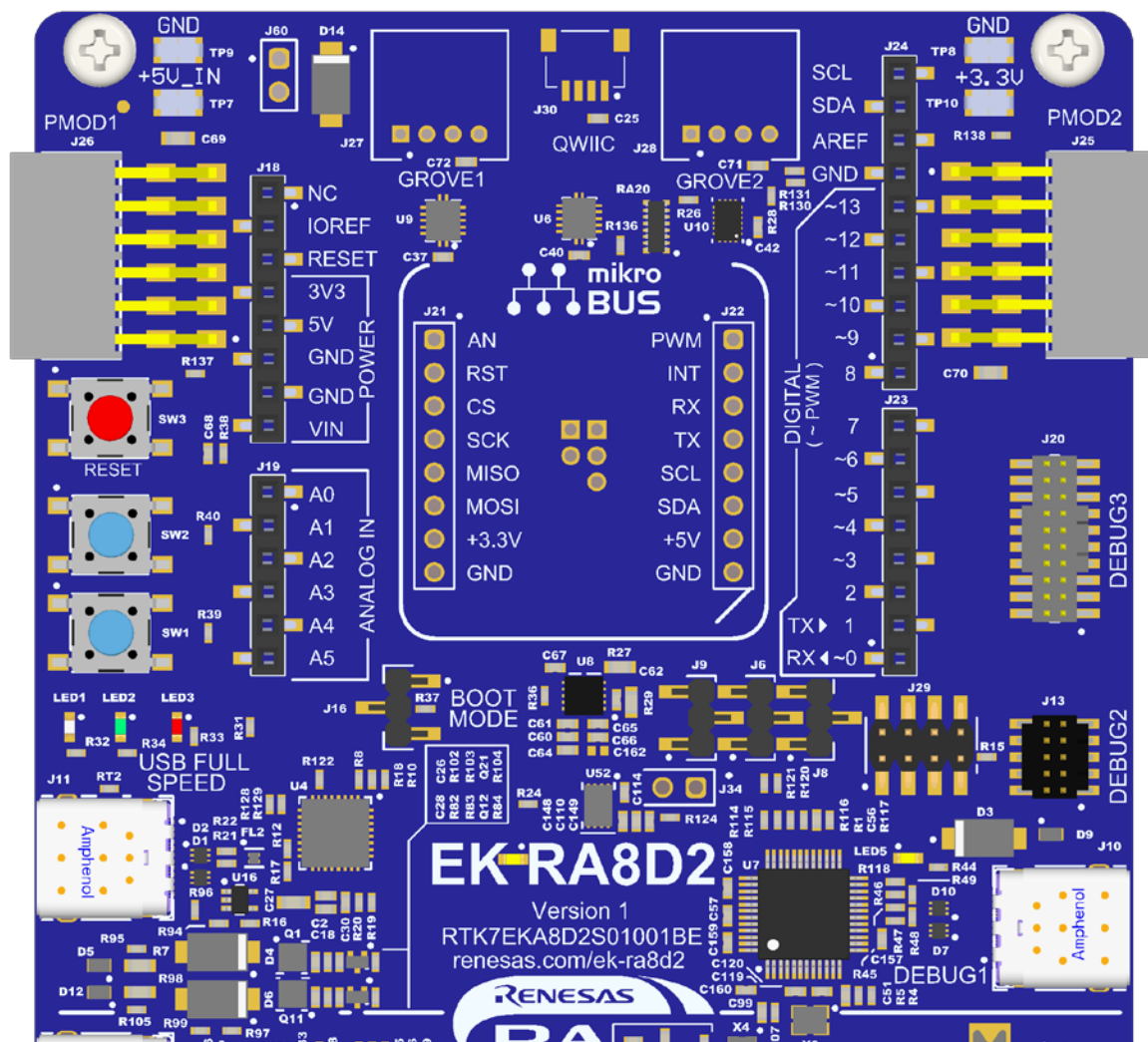
Figure 7. System Control and Ecosystem Access Area
