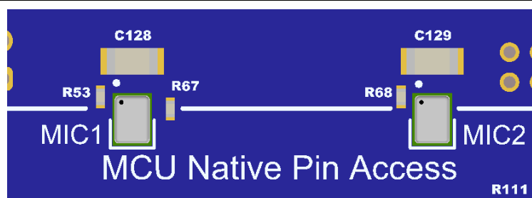
Figure 29. MEMS Microphones
