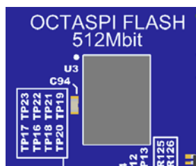
Figure 27. Octo-SPI Flash (labelled as “OCTASPI” on silkscreen text)
