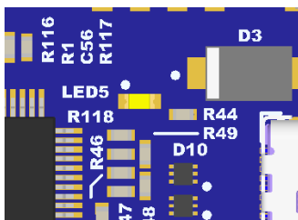
Figure 20. Debug LED
