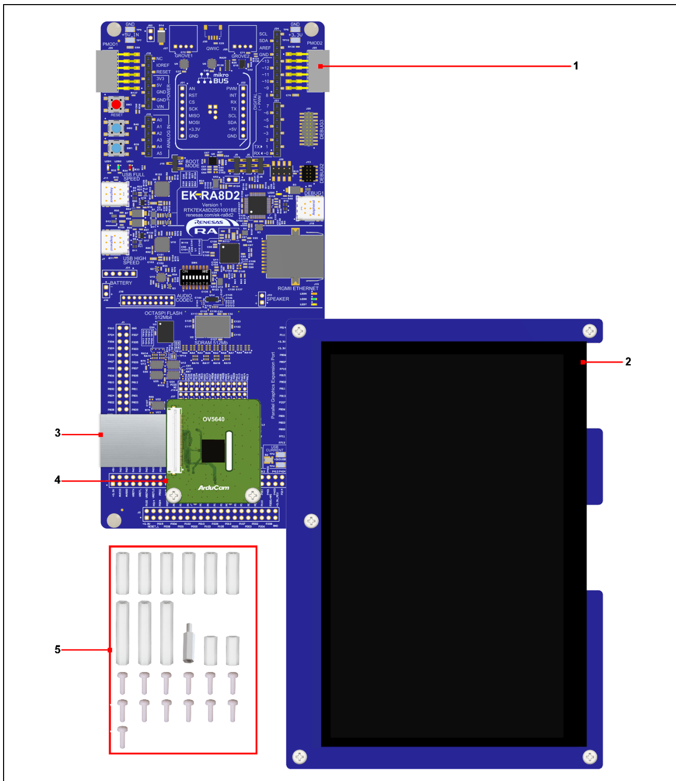
Figure 3. EK-RA8D2 Kit Contents
