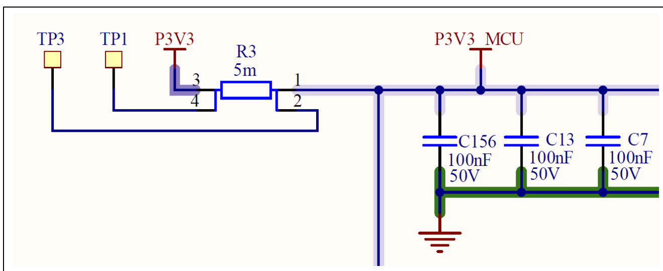
Figure 33. RA +3.3 V Current Measurement Circuit
