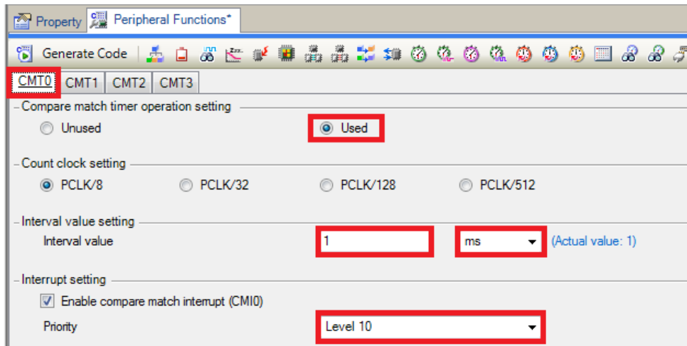
Figure 4-7 CMT0 tab
