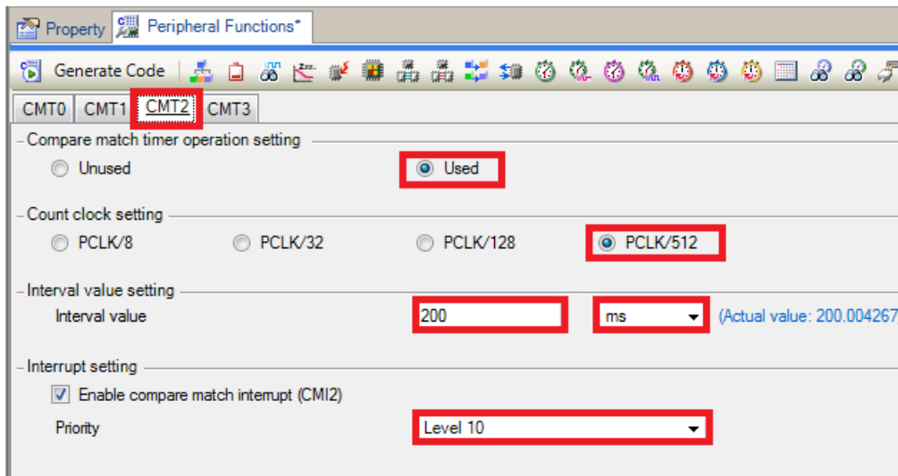
Figure 4-9 CMT2 tab
