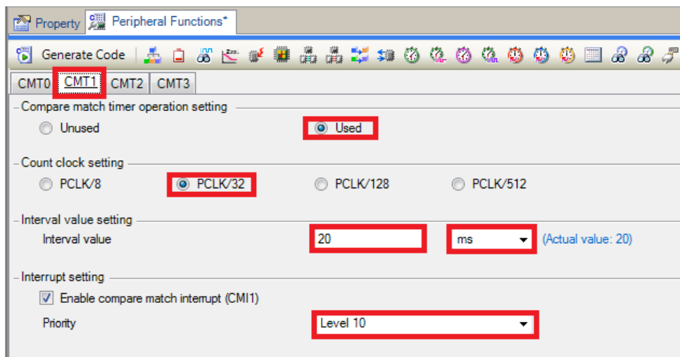
Figure 4-8 CMT1 tab
