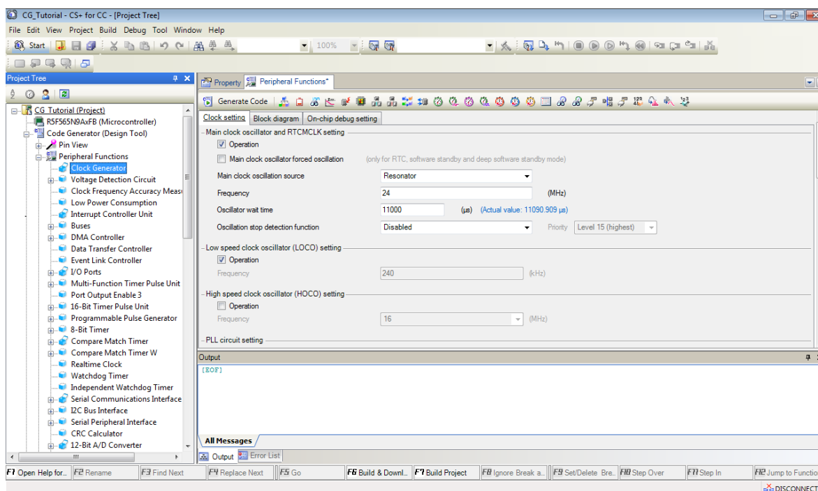
Figure 4-1 Initial View
