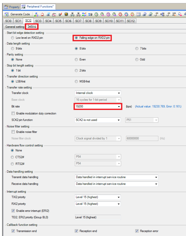
Figure 4-17 SCI2 Setting tab
