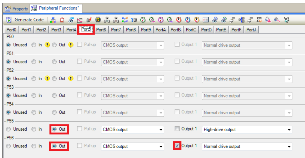
Figure 4-23 I/O ports – Port5
