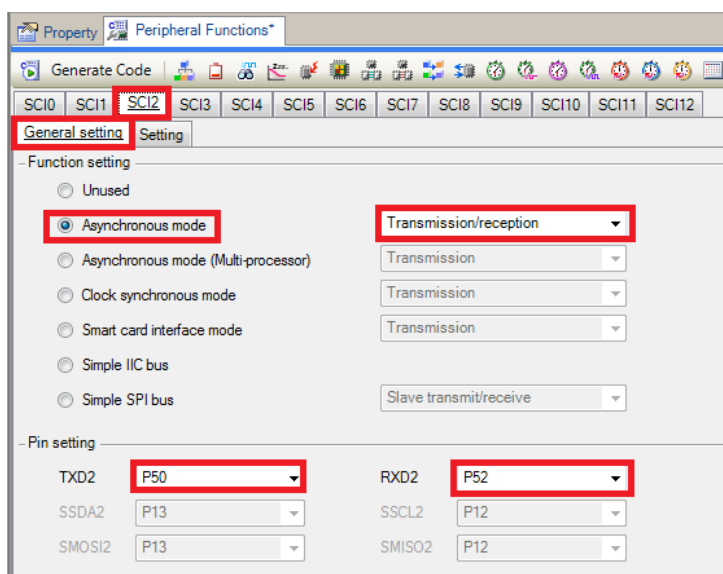
Figure 4-16 SCI2 General Setting tab
