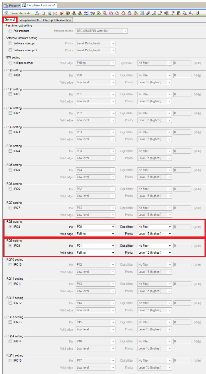
Figure 4-4 Interrupt Functions tab
