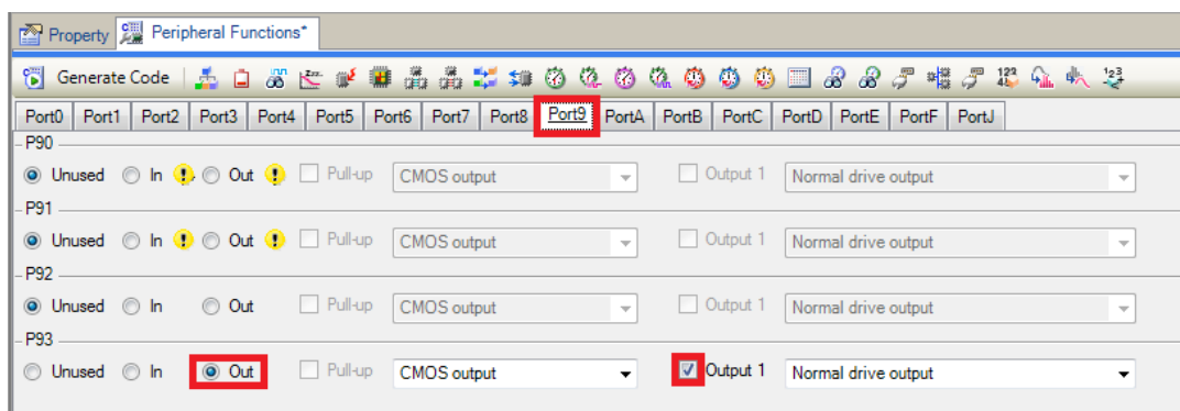
Figure 4-24 I/O ports – Port9
