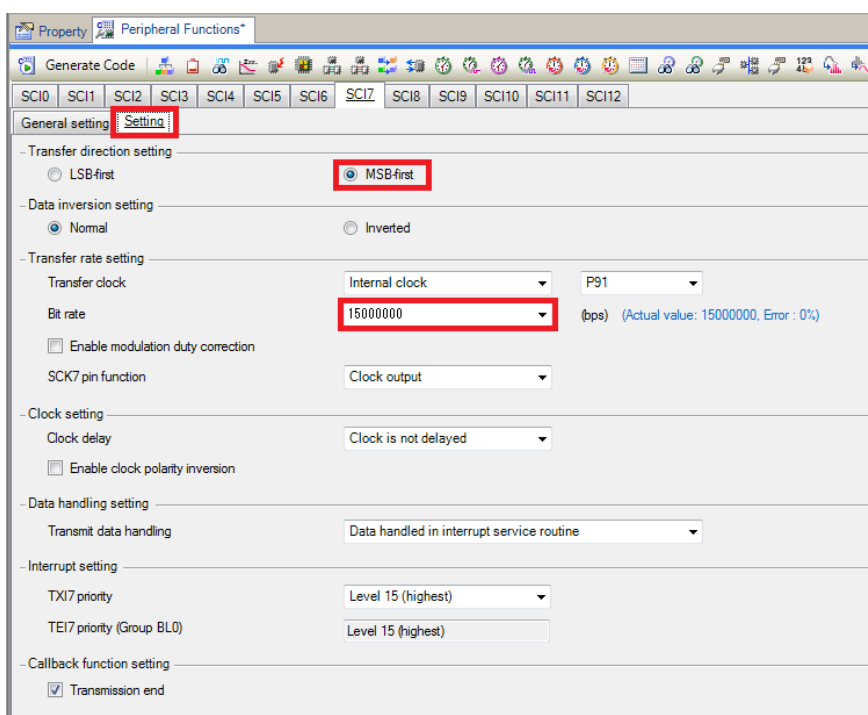
Figure 4-15 SCI7 Setting tab
