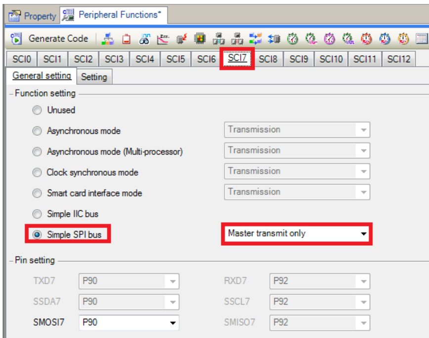
Figure 4-14 SCI7 General Setting tab
