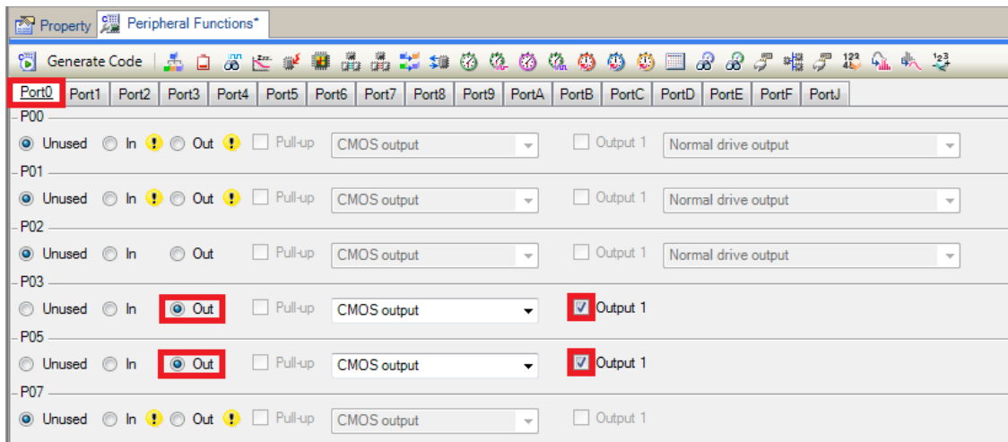
Figure 4-19 I/O ports – Port0
