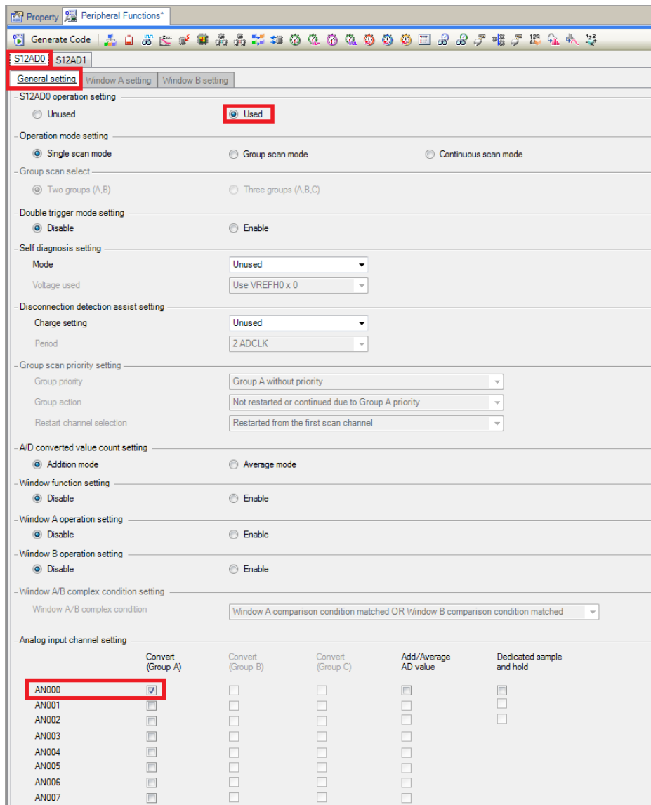
Figure 4-11 S12AD0 tab (1)
