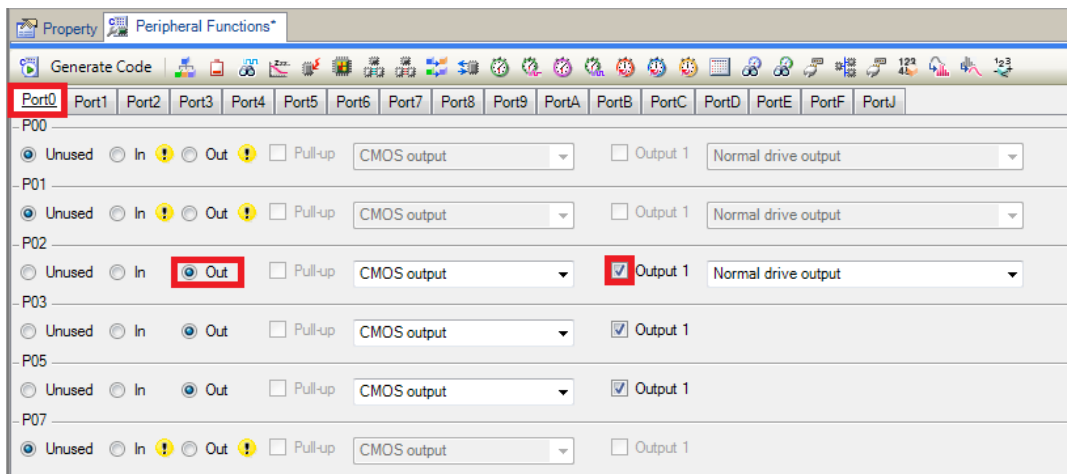
Figure 4-22 I/O ports – Port0
