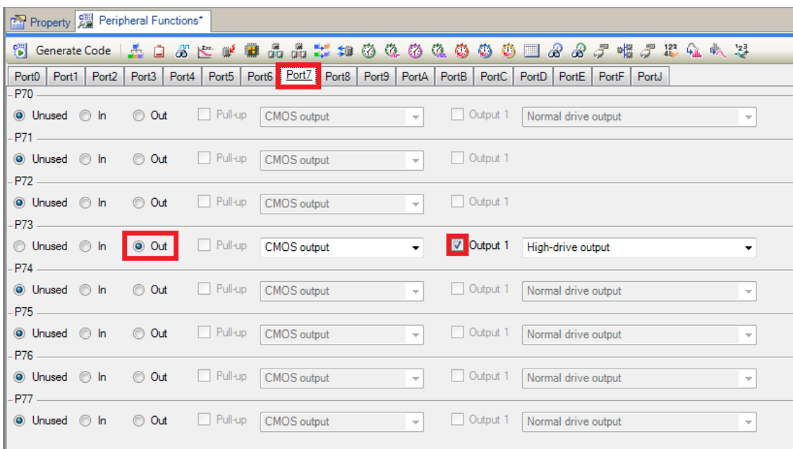
Figure 4-20 I/O ports – Port7
