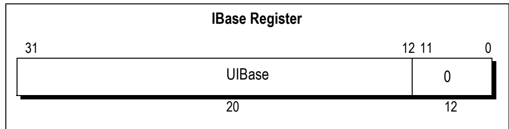
Figure 6.10 IBase Register
