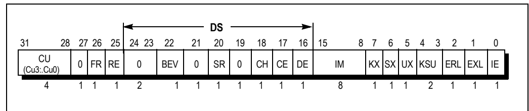
Figure 3.4 Status Register (4600/4700)
