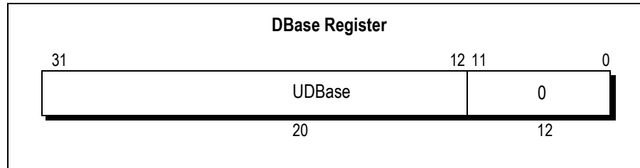
Figure 6.12 DBase Register
