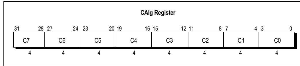
Figure 6.14 CAIlg Register
