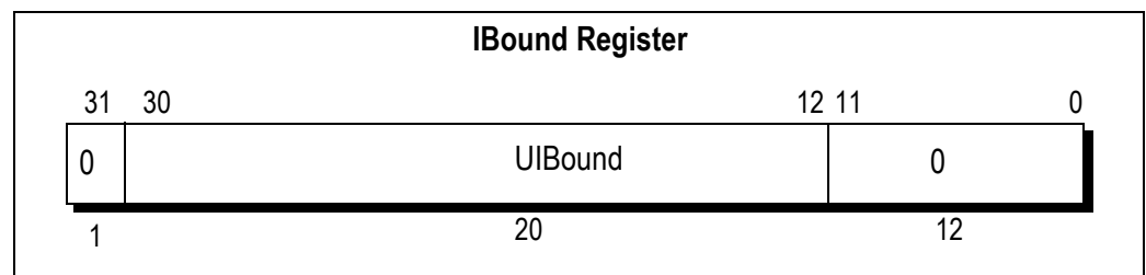
Figure 6.11 IBound Register
