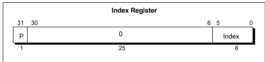
Figure 6.4 Index Register
