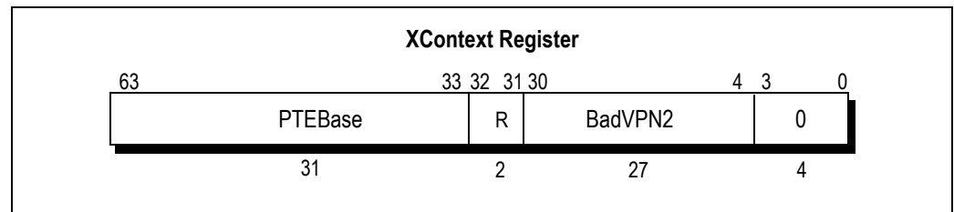
Figure 3.12 XContext Register Format
