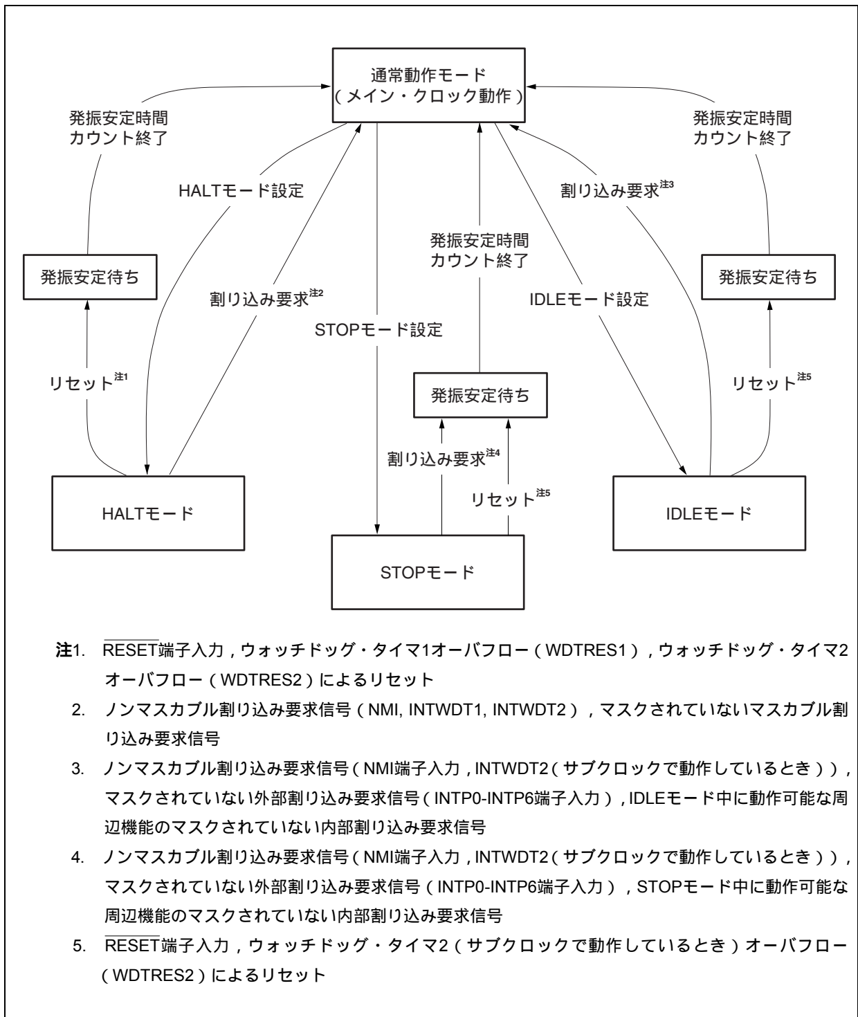
図21-1 状態遷移図 (1/2)
