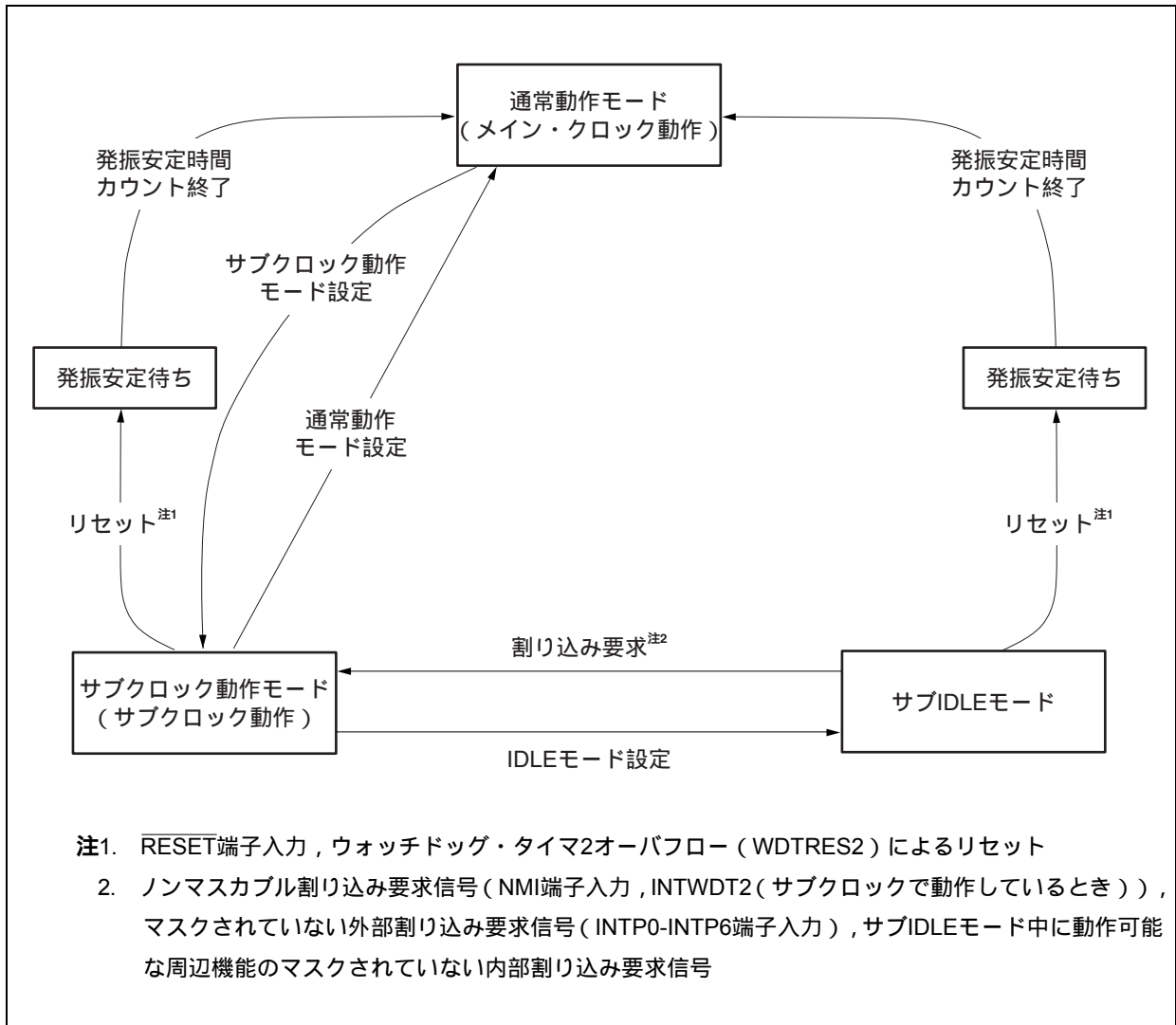
図21-1 状態遷移図 (2/2)
