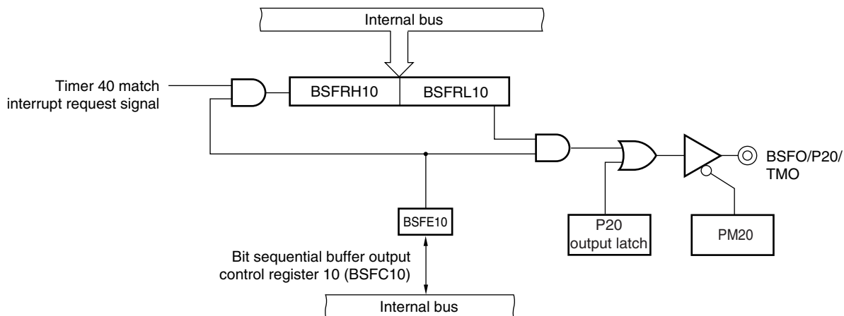
Figure 12-1. Block Diagram of Bit Sequential Buffer
