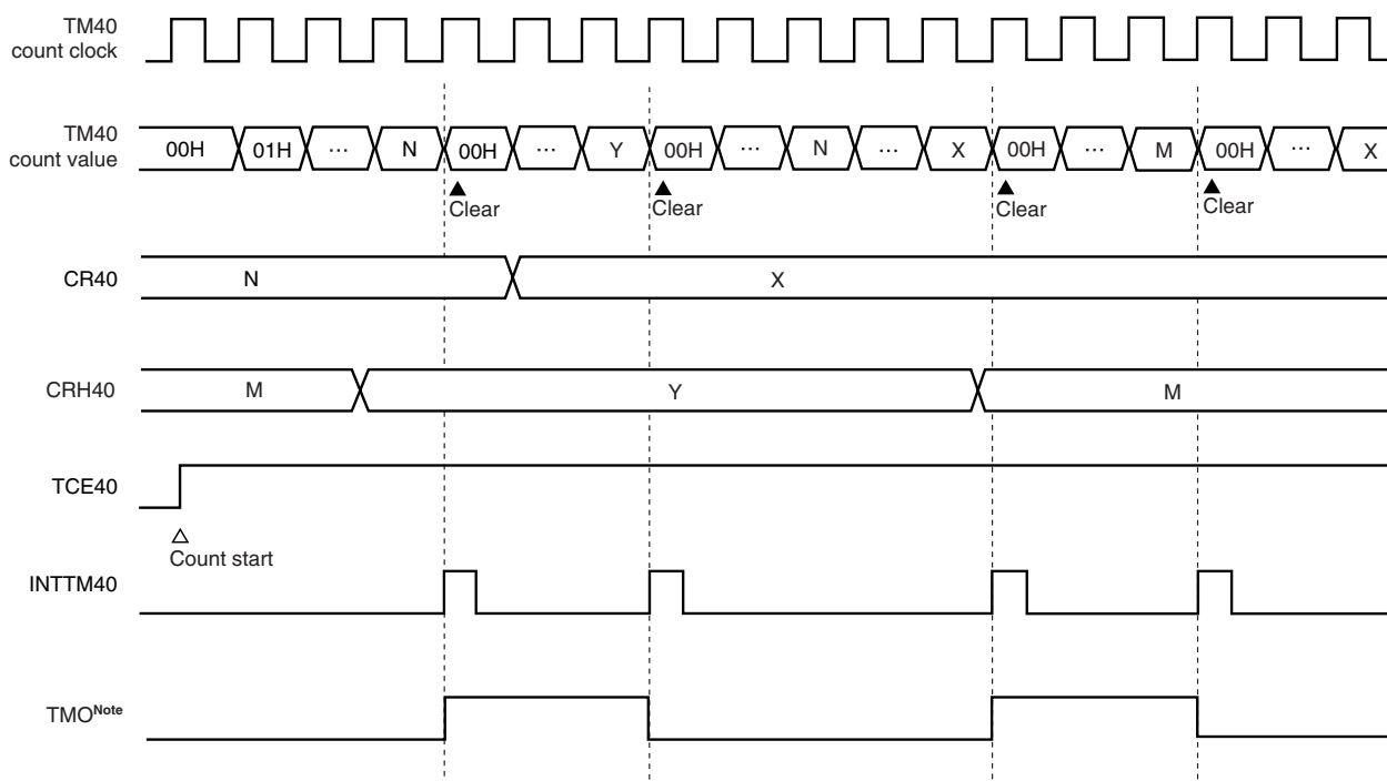
Figure 9-23. PWM Output Mode Timing (When CR40 and CRH40 Are Overwritten)
