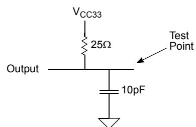
Figure 45: PCI T_{OV(max)} Falling Edge AC Test Load
