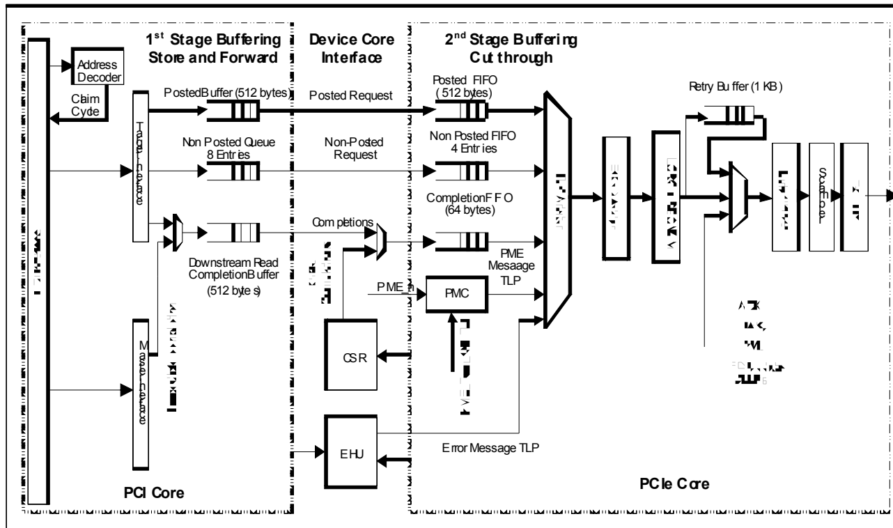
Figure 6: Upstream Data Path
