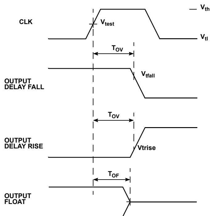
Figure 43: Output Timing Measurement Waveforms
