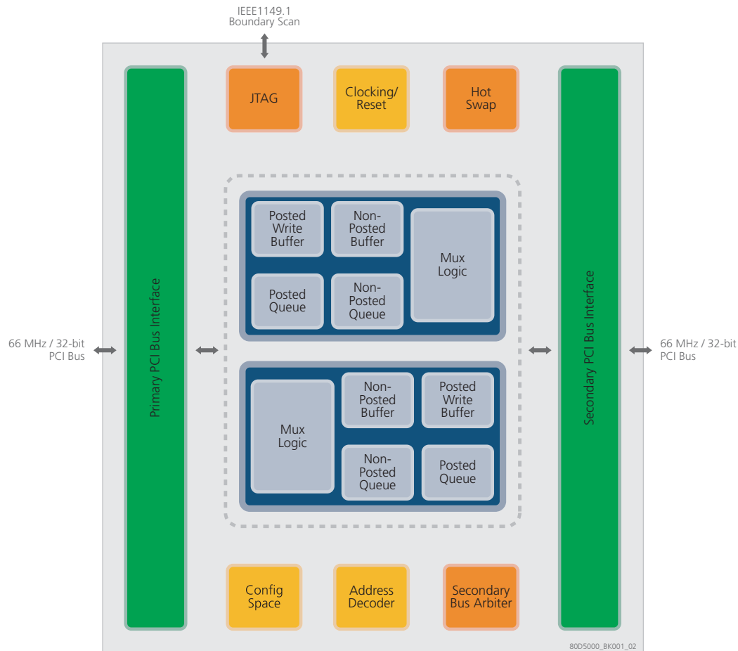
Figure 1: Block Diagram
