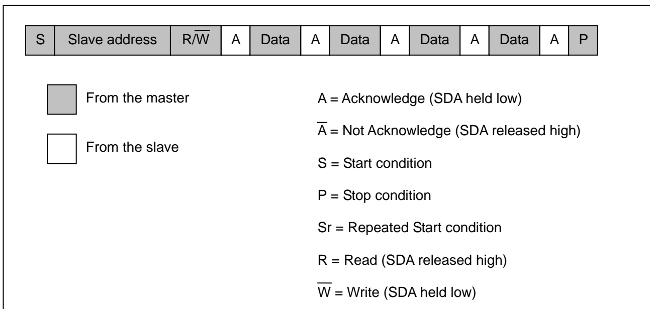
Figure 5-43: I 2 C bus activity notation
