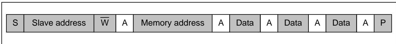
Figure 5-44: The bus activity, showing 4 bytes being transmitted to the EEPROM
