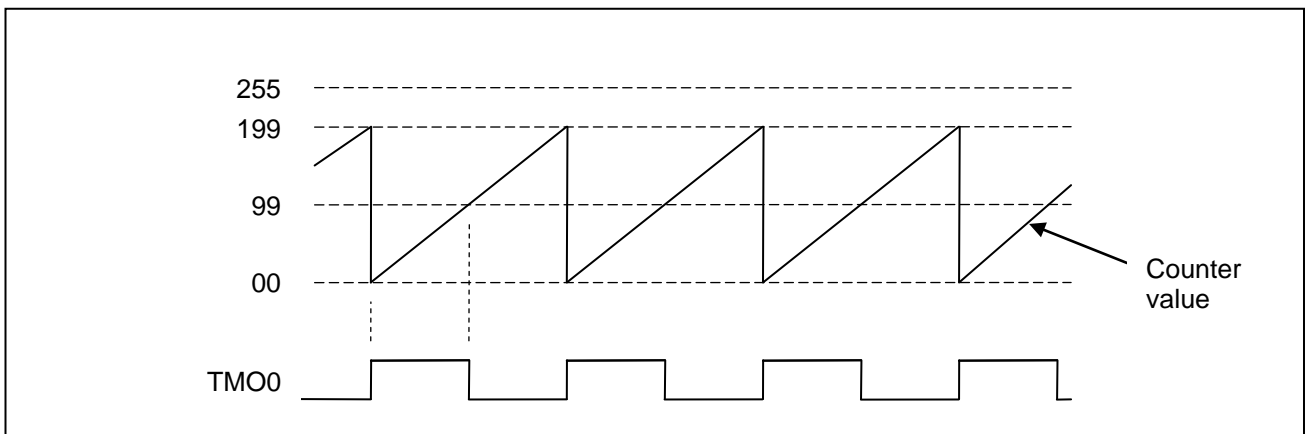
Figure 5-20: Example of pulse output operation
