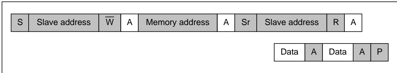
Figure 5-48: The bus activity, showing the Repeated Start condition when switching to the Read process
