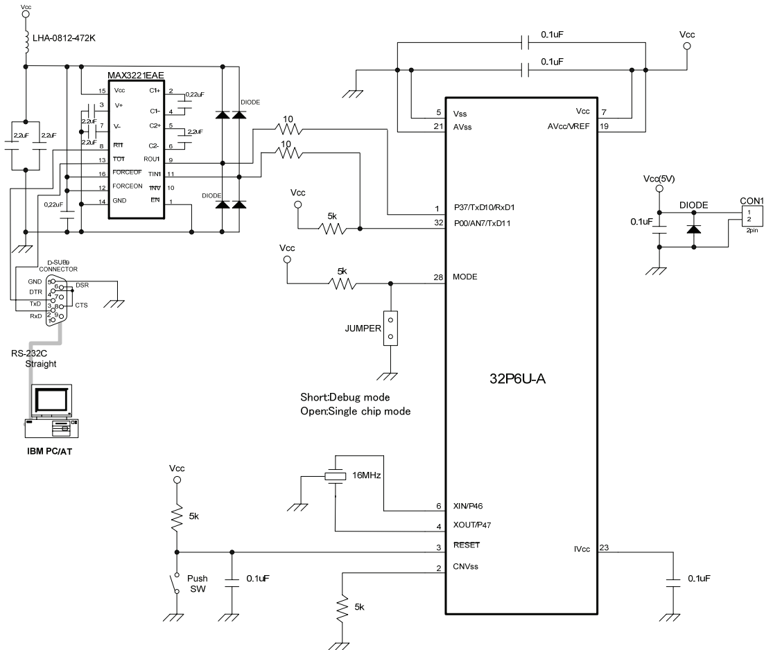
Figure 2 Circuit Example with RS-232C Cable
