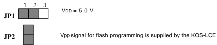
Figure 2-2. Default Jumper Settings
