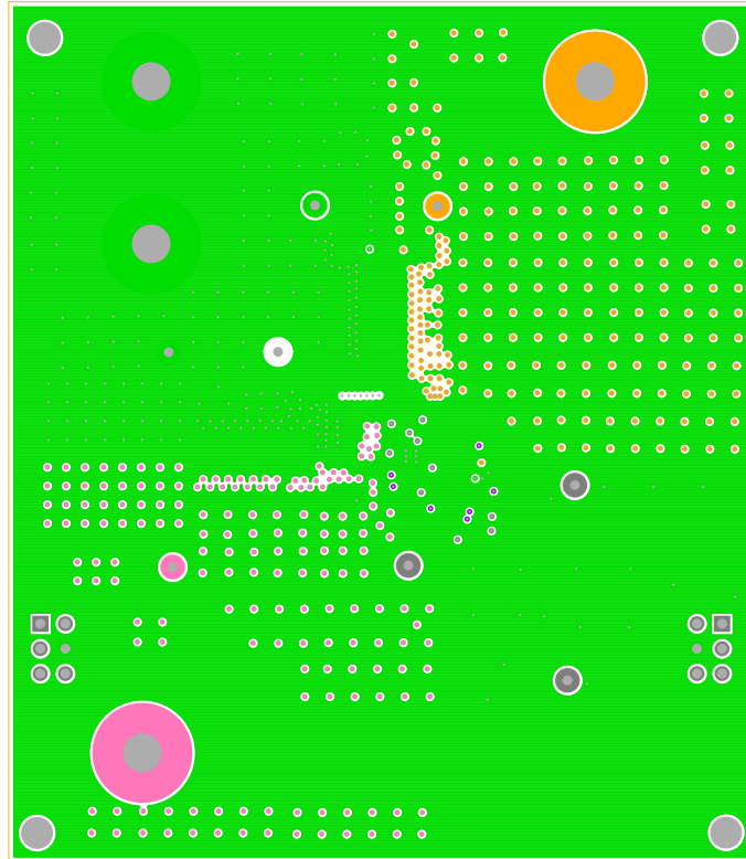
Figure 12. Inner Layer 5
