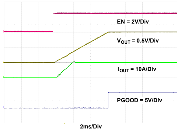
Figure 22. Startup Waveform at I_{OUT} = 10A
