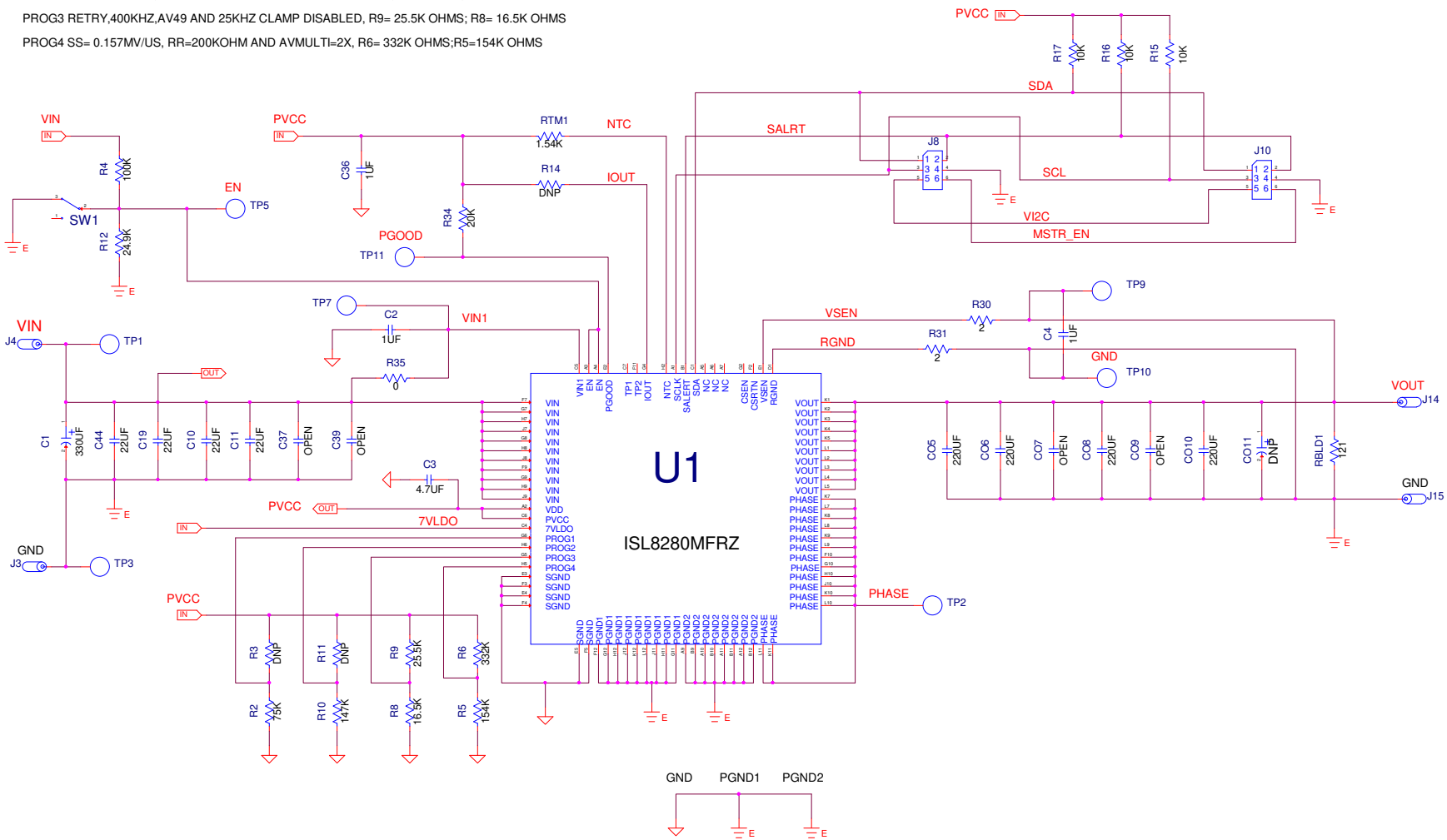
Figure 6. Schematic
