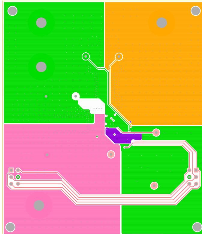
Figure 10. Inner Layer 3
