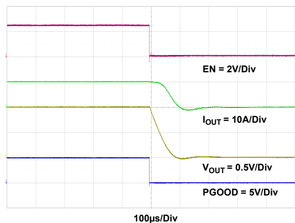
Figure 24. Shutdown Waveform at I_{OUT} = 10A
