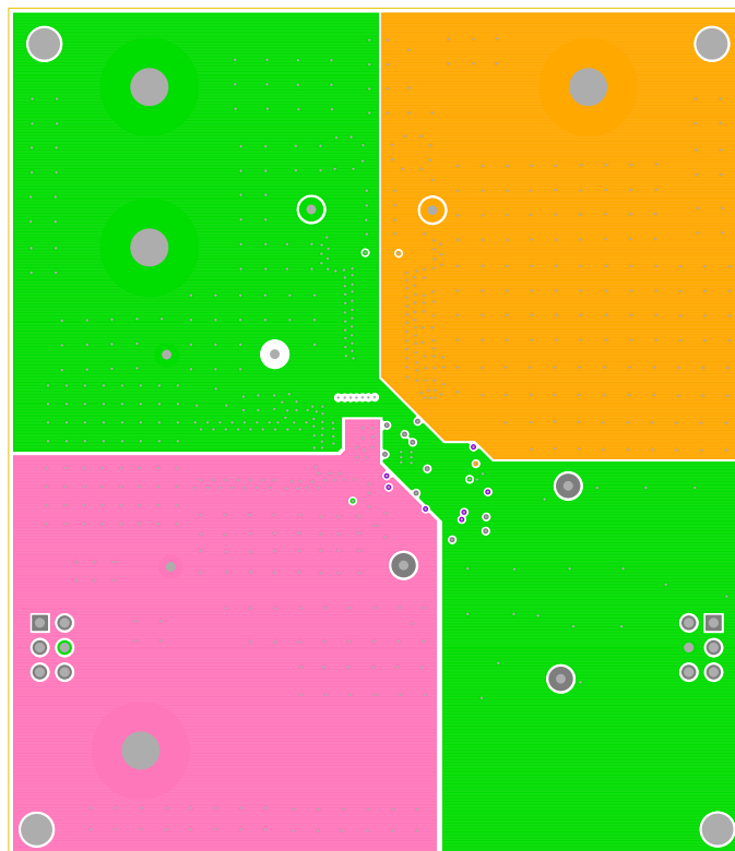
Figure 11. Inner Layer 4
