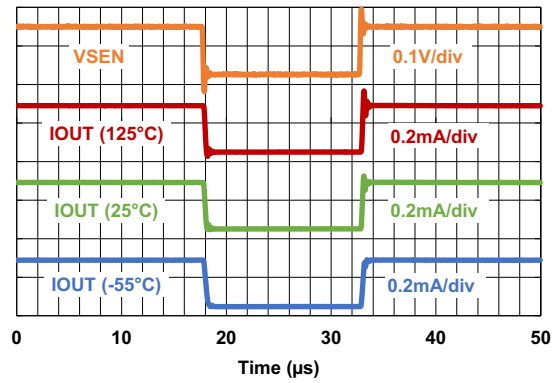
Figure 21. Input Step Response
