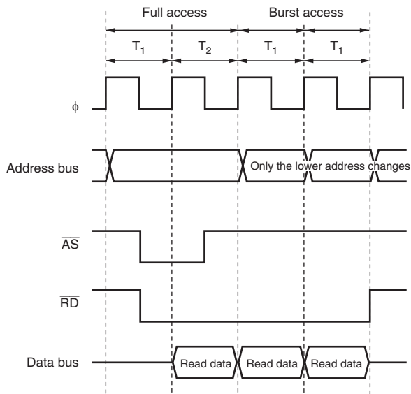
Figure 7.15 Example of Burst ROM Access Timing ( AST0 = 0 and BRSTS1 = 0 )
