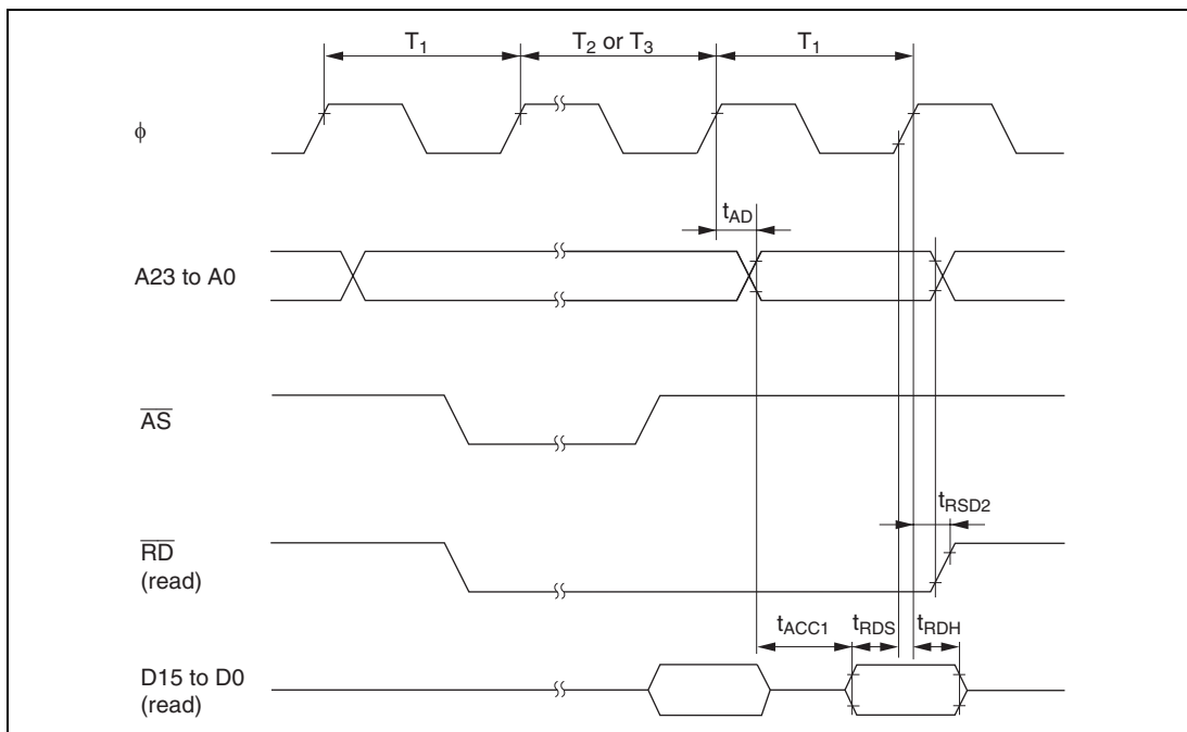
Figure 21.10 Burst ROM Access Timing (Two-State Access)
