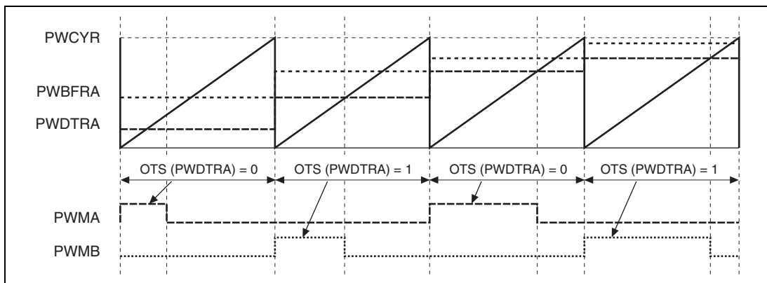
Figure 15.7 PWM Operation
