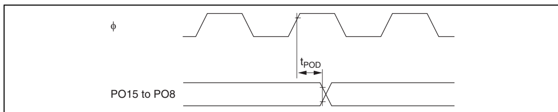
Figure 21.12 PPG Output Timing
