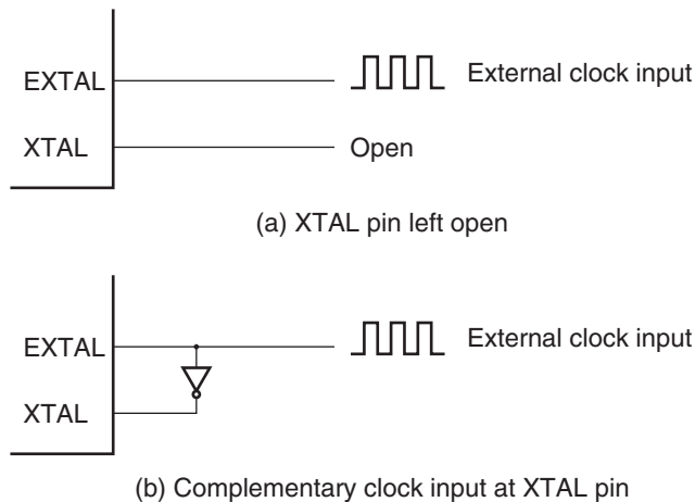
Figure 18.4 External Clock Input (Examples)
