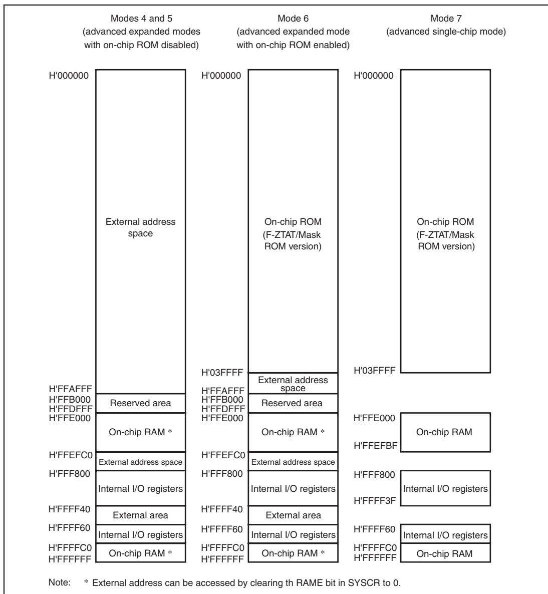
Figure 3.1 Address Map (H8S/2609)
