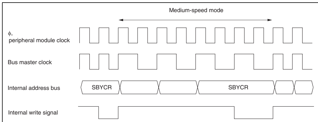
Figure 19.2 Medium-Speed Mode Transition and Clearance Timing
