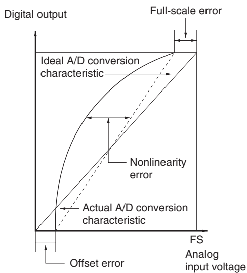
Figure 14.5 A/D Conversion Accuracy Definitions
