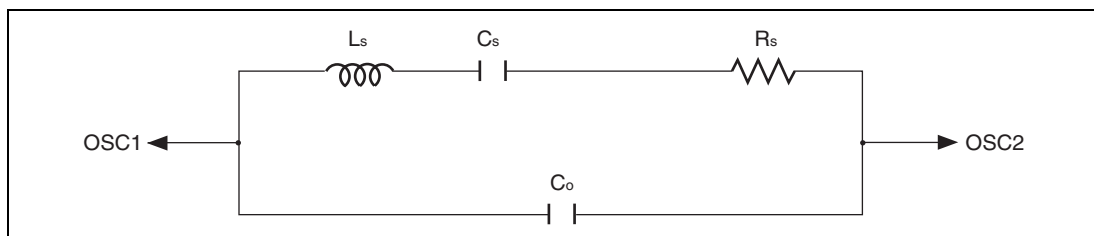
Figure 18.7 Equivalent Circuit for 32.768-kHz Crystal Resonator
