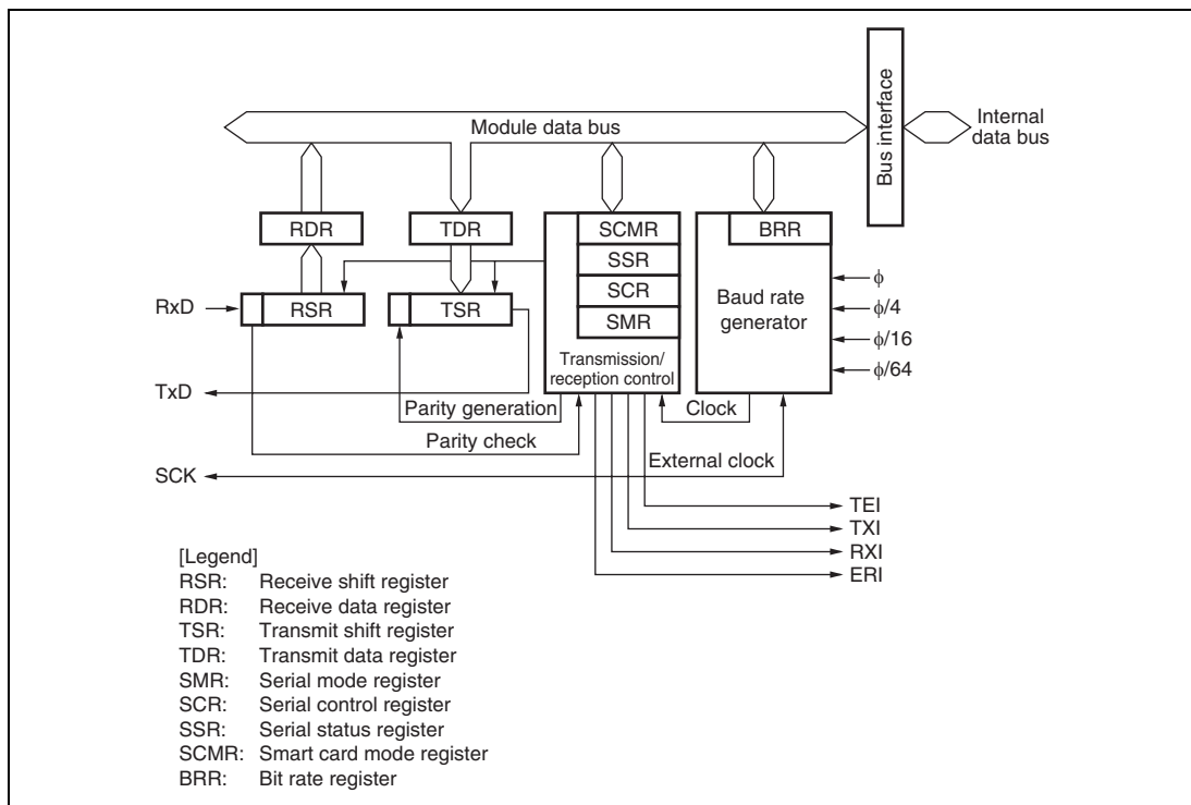
Figure 13.1 Block Diagram of SCI
