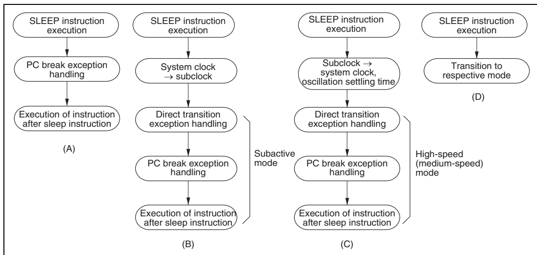
Figure 6.2 Operations in Power-Down Mode Transitions
