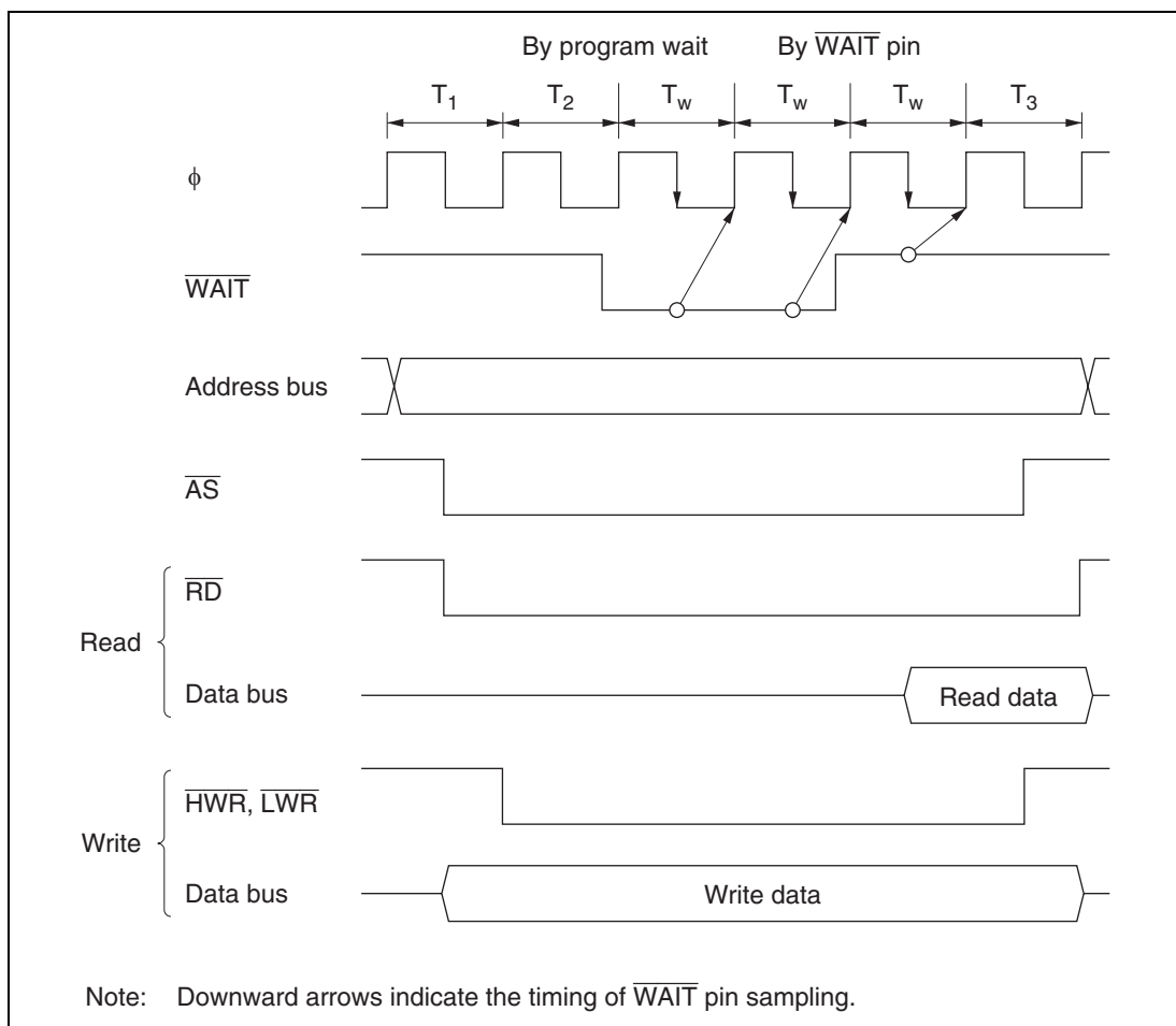
Figure 7.13 Example of Wait State Insertion Timing
