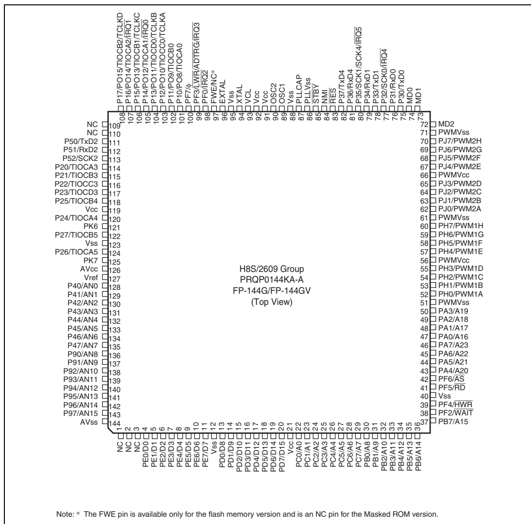
Figure 1.2 Pin Assignments
