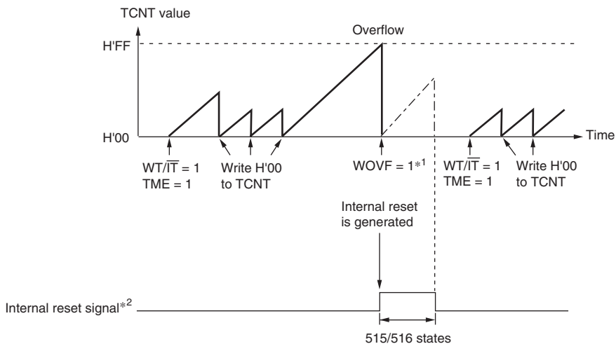
Figure 12.3 (a) WDT_0 Operation in Watchdog Timer Mode
