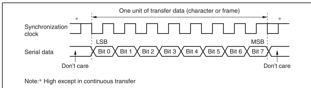
Figure 13.14 Data Format in Synchronous Communication (For LSB-First)
