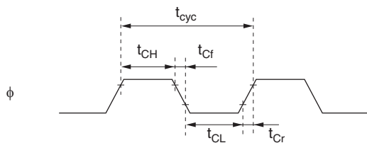
Figure 21.2 System Clock Timing
