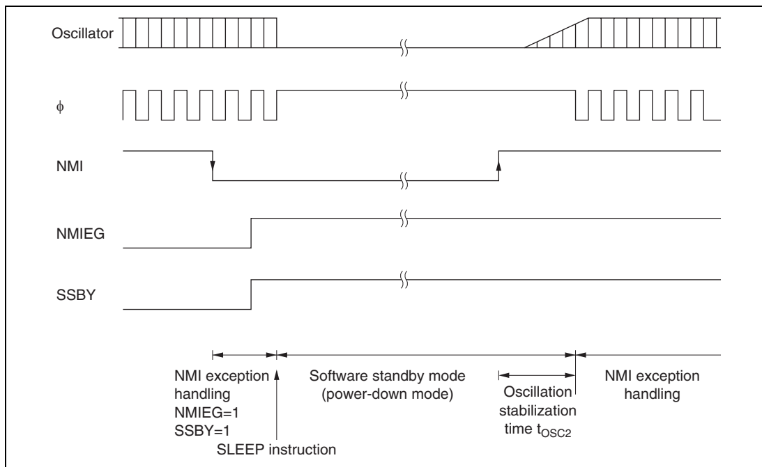
Figure 19.3 Software Standby Mode Application Example
