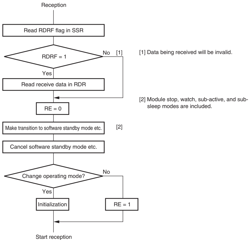
Figure 13.37 Sample Flowchart for Mode Transition during Reception
