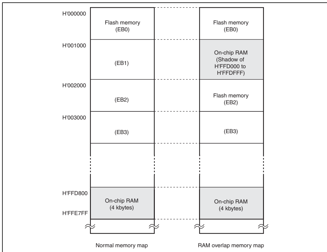
Figure 17.8 Example of RAM Overlap Operation
