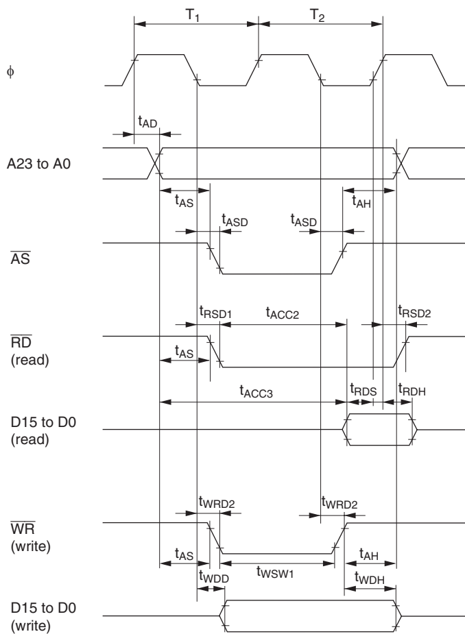
Figure 21.6 Basic Bus Timing (Two-State Access)
