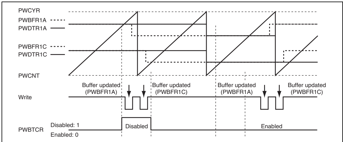
Figure 15.8 Disabling Buffer Transfer
