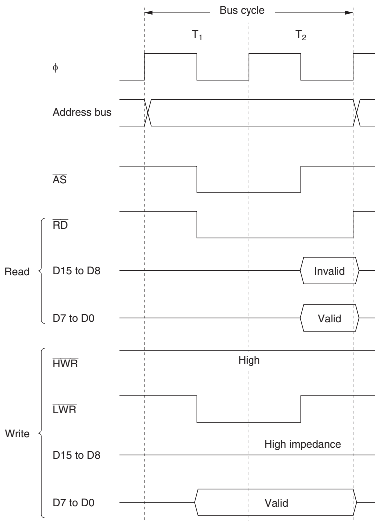
Figure 7.8 Bus Timing for 16-Bit, 2-State Access Space (Odd Address Byte Access)
