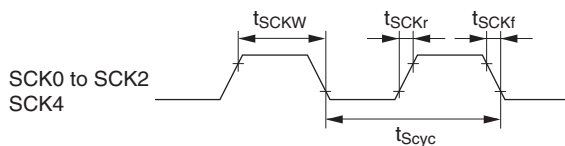
Figure 21.16 SCK Clock Input Timing
