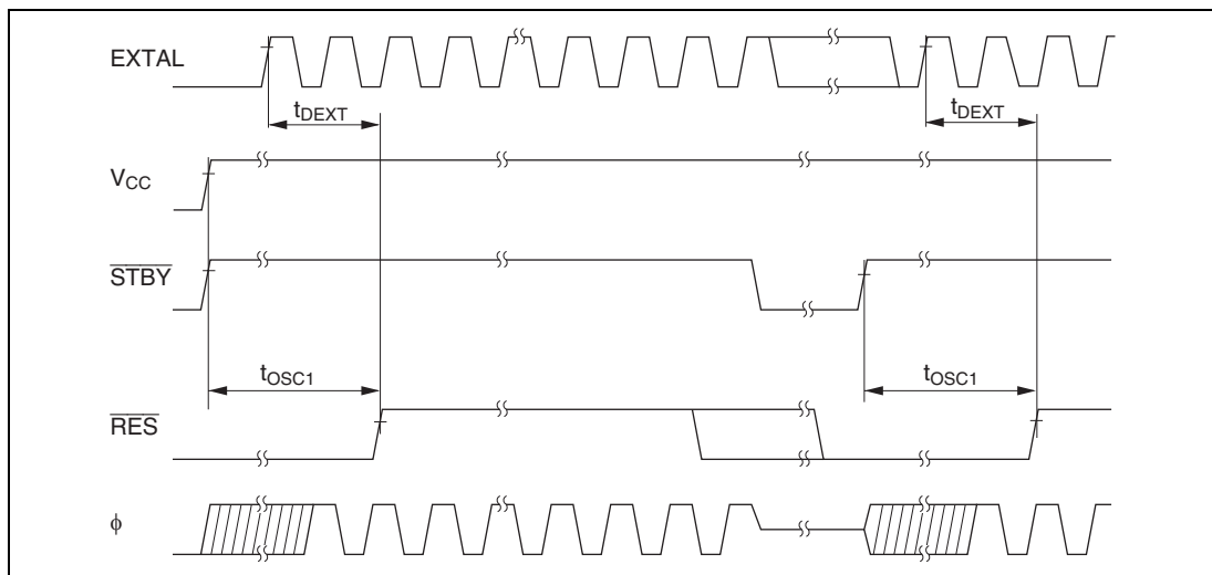
Figure 21.3 Oscillator Settling Timing
