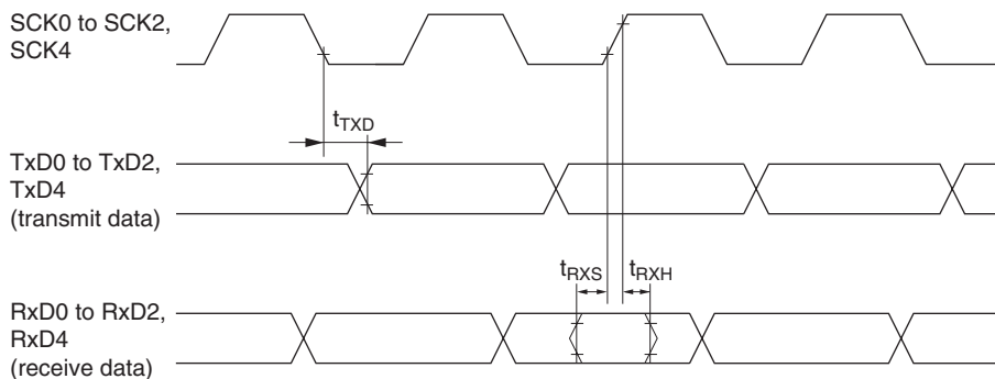
Figure 21.17 SCI Input/Output Timing (Clock Synchronous Mode)
