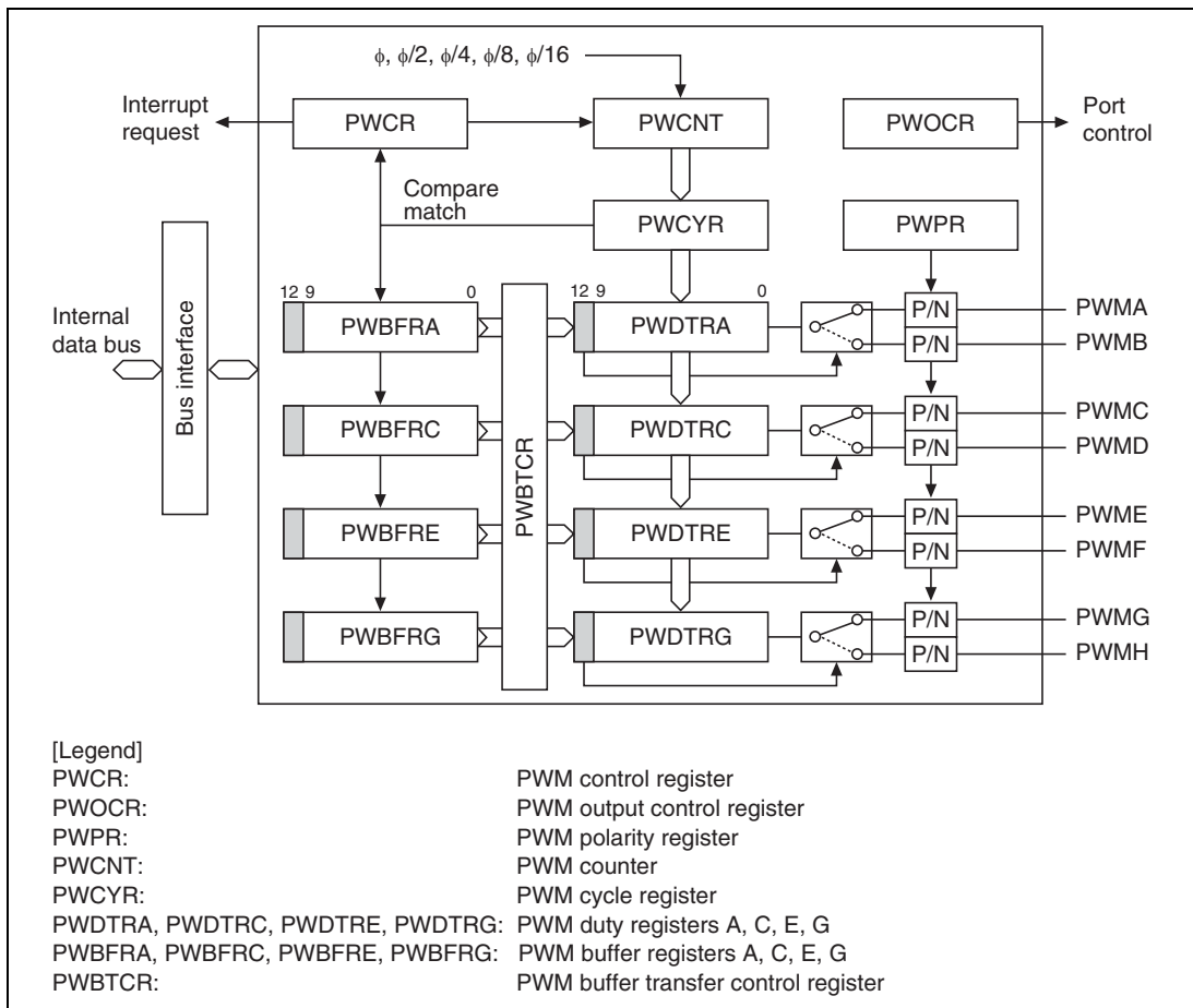
Figure 15.1 Block Diagram of PWM
