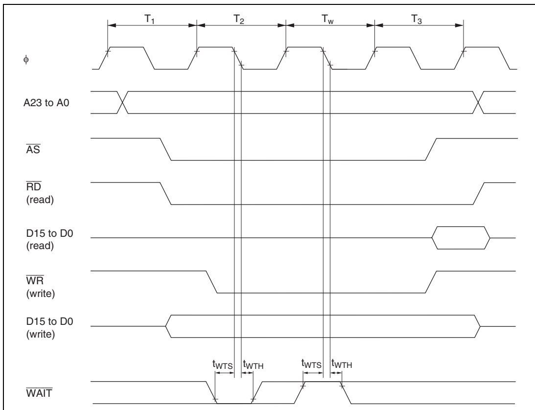
Figure 21.8 Basic Bus Timing (Three-State Access with One Wait State)
