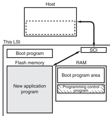
Figure 17.3 Boot Mode
