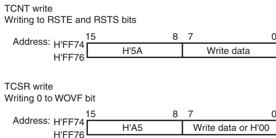
Figure 12.4 Writing to TCNT, TCSR, and RSTCSR (example for WDT0)
