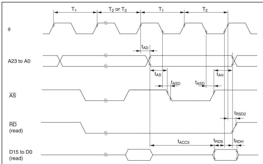
Figure 21.9 Burst ROM Access Timing (Two-State Access)
