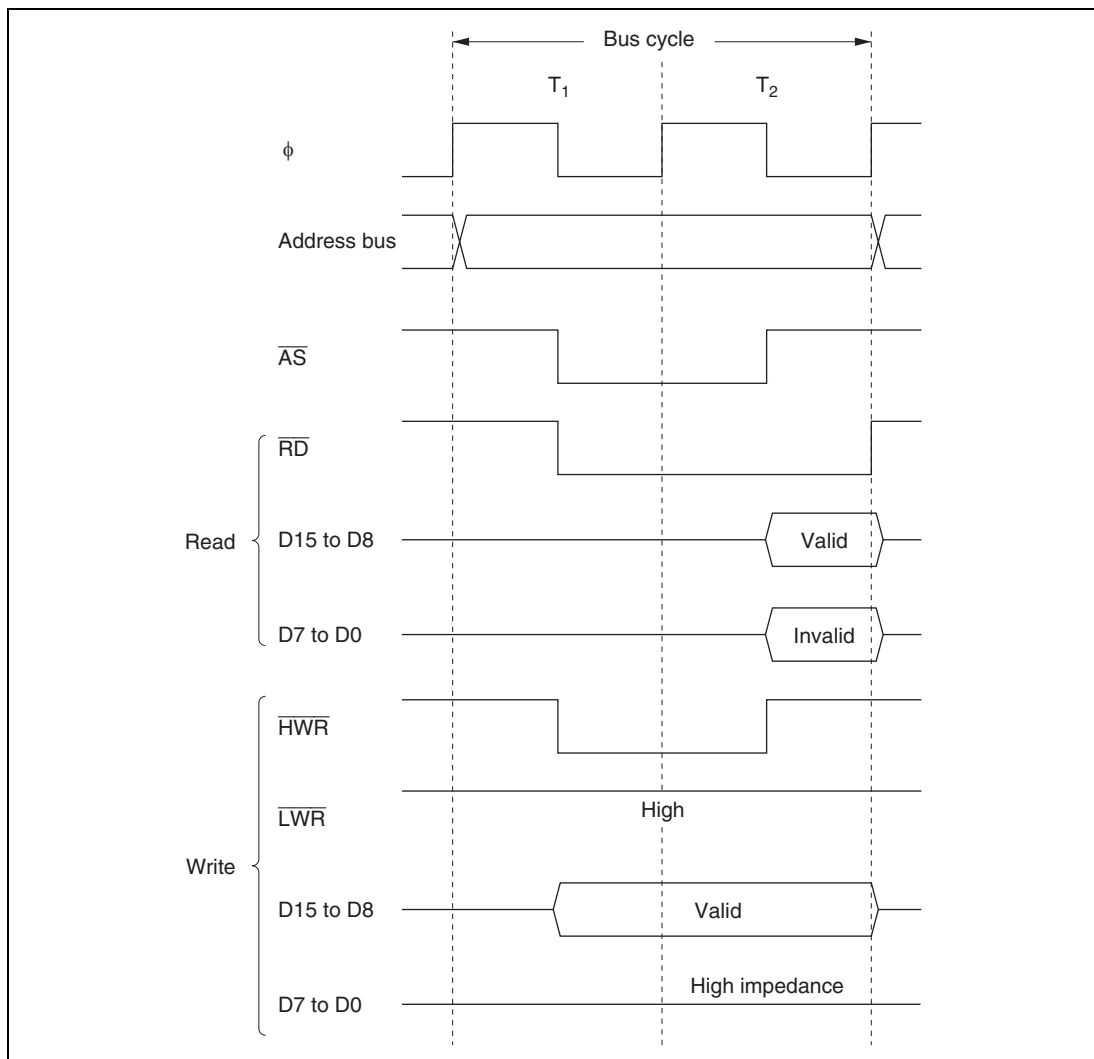
Figure 7.5 Bus Timing for 8-Bit, 2-State Access Space
