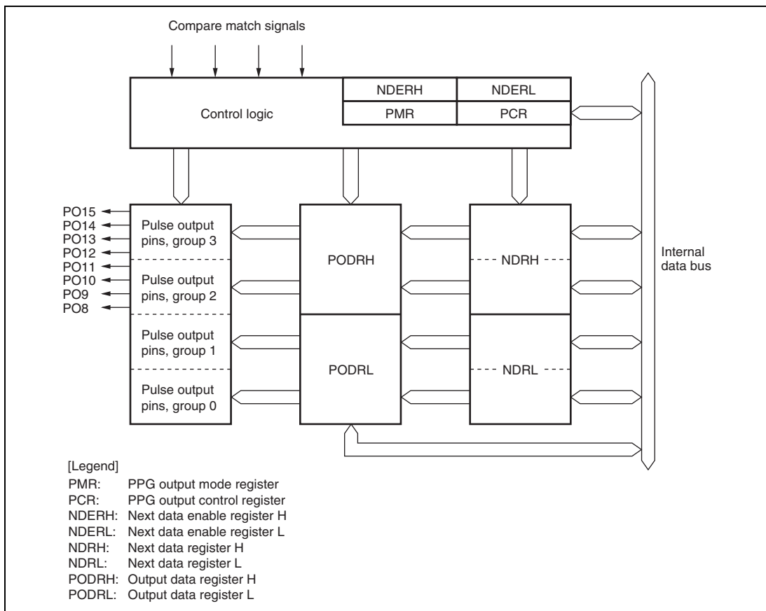
Figure 11.1 Block Diagram of PPG
