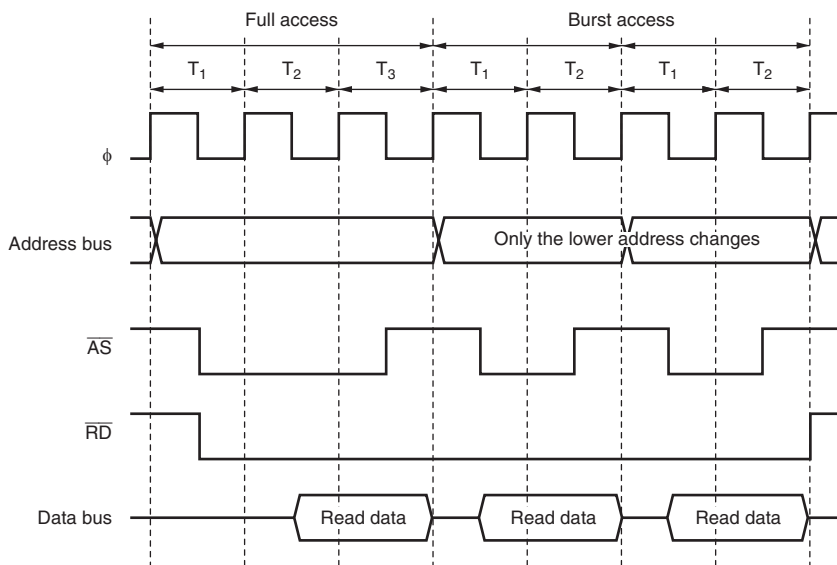
Figure 7.14 Example of Burst ROM Access Timing ( AST0 = 1 and BRSTS0 = 1 )
