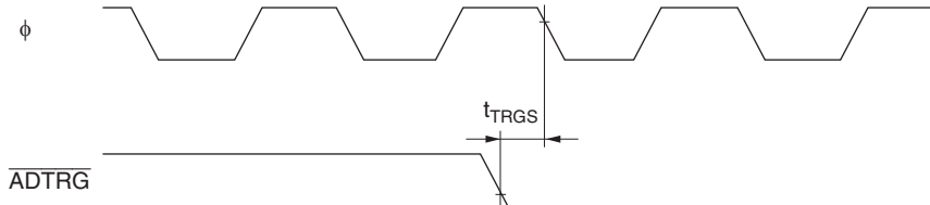
Figure 21.18 A/D Converter External Trigger Input Timing
