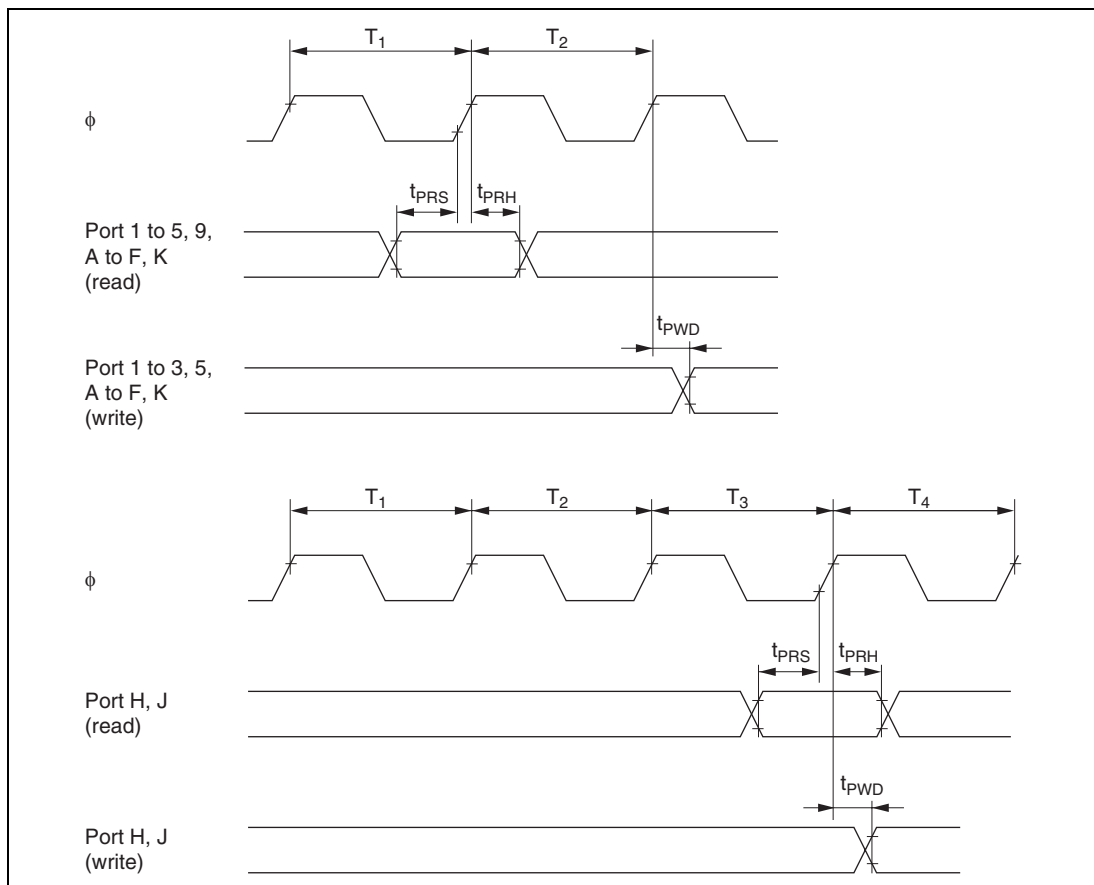
Figure 21.11 I/O Port Input/Output Timing
