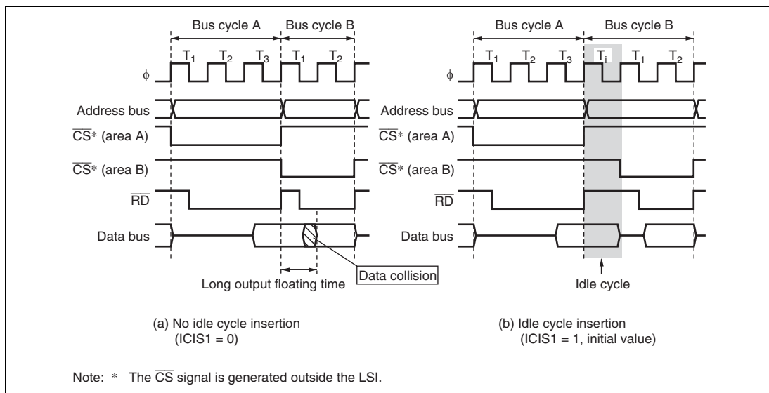
Figure 7.16 Example of Idle Cycle Operation (Consecutive Reads in Different Areas)
