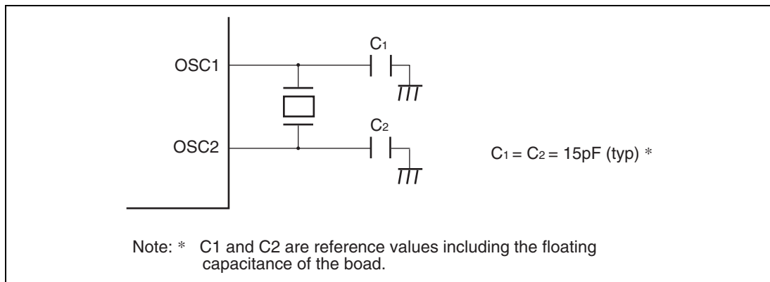
Figure 18.6 Connection Example of 32.768-kHz Crystal Resonator
