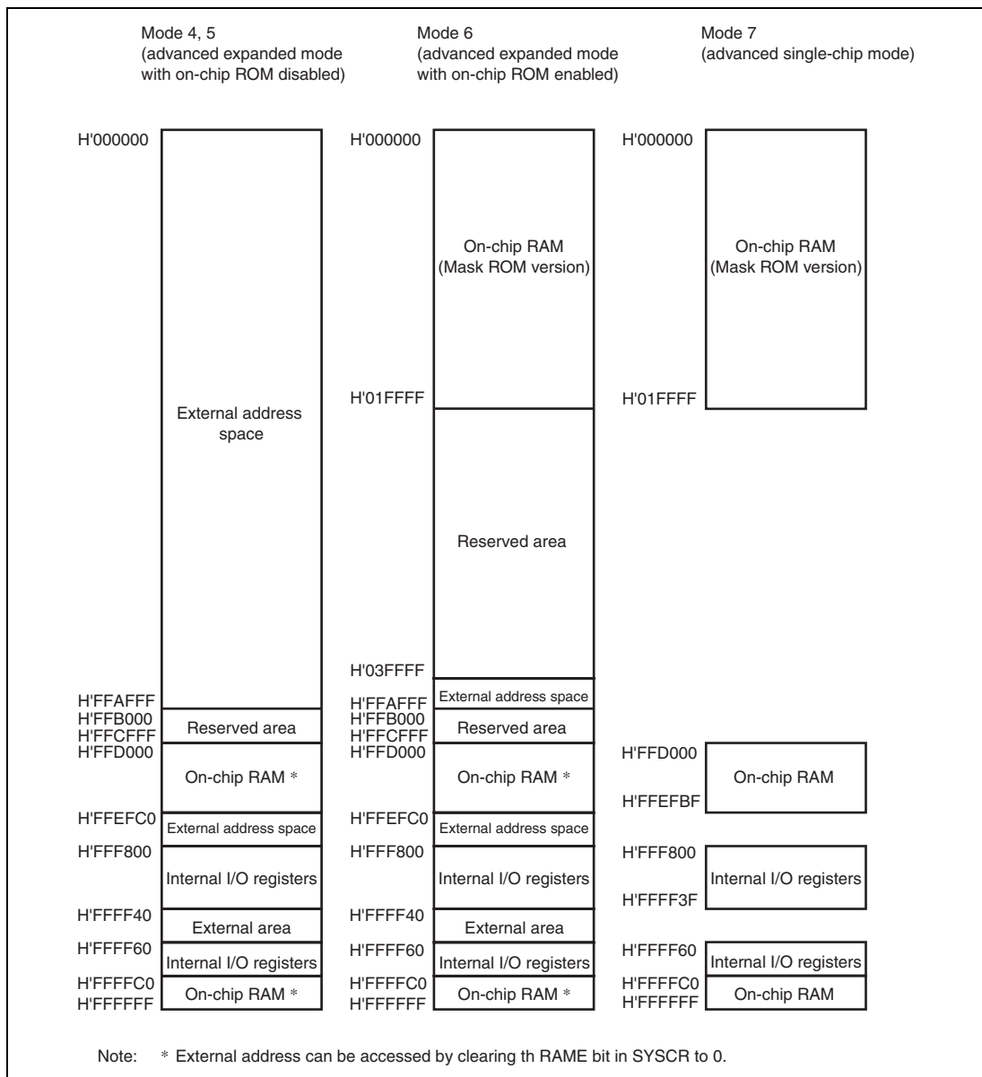
Figure 3.2 Address Map (H8S/2608)
