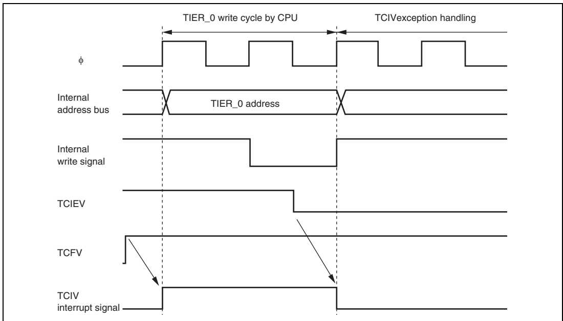
Figure 5.6 Conflict between Interrupt Generation and Disabling
