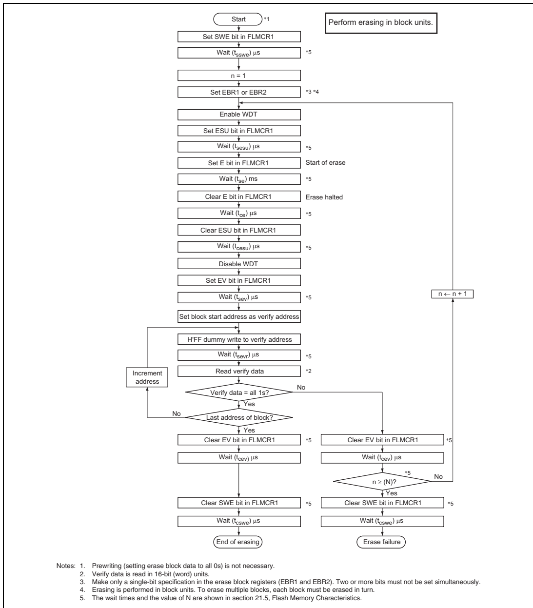
Figure 17.10 Erase/Erase-Verify Flowchart
