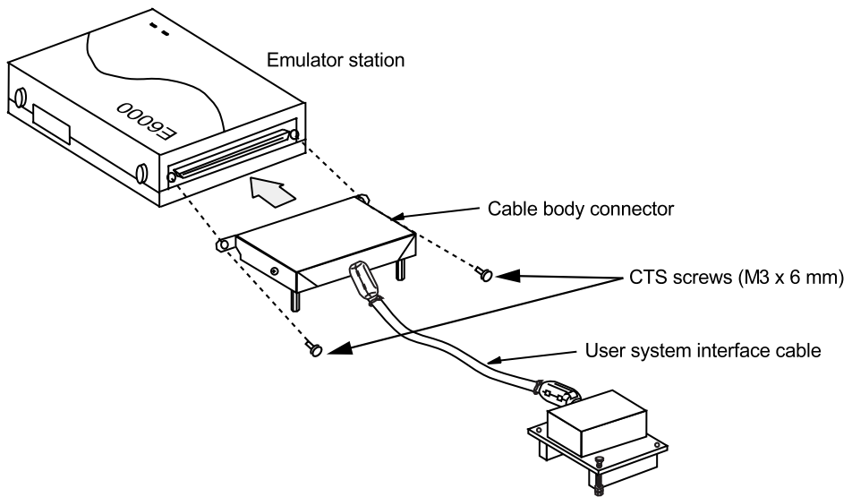
Figure 2 Connecting User System Interface Cable to Emulator Station
